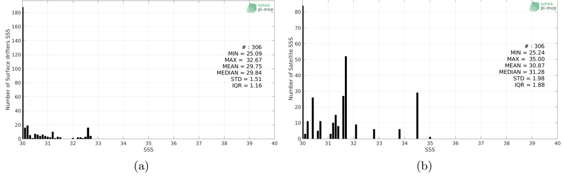
Figure 2: Histograms of SSS from Surface drifters (a) and SMOS L4 v2 Weekly (CATDS-CECOS-IFREMER) (b) considering all match-up pairs per bins of 0.1 over the Bay of Bengal Pi-MEP region and for the full satellite product period.
