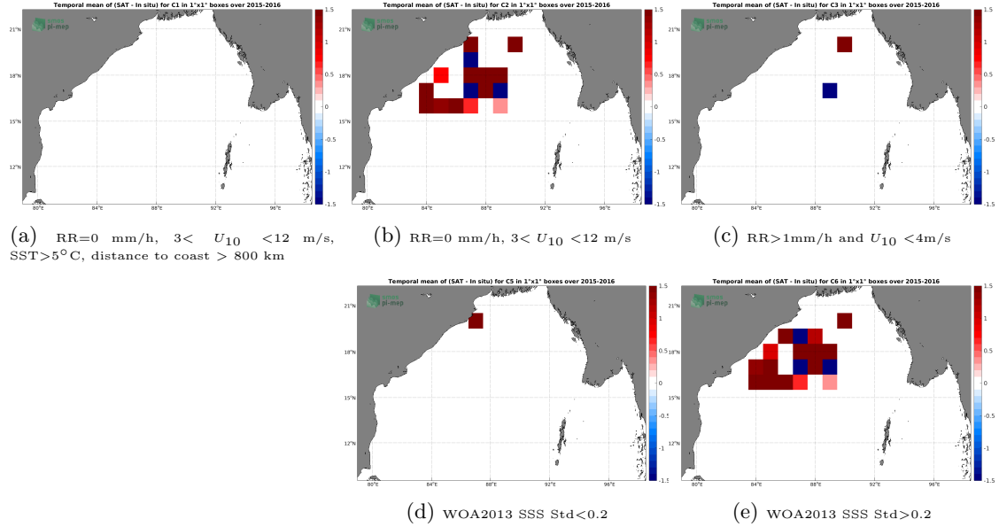
Figure 11: Temporal mean gridded over spatial boxes of size 1^{\circ}\times 1^{\circ} of \Delta\text{SSS} (SMOS L4 v2 Weekly (CATDS-CECOS-IFREMER) - Surface drifters) for 5 different subdatasets corresponding to: RR=0 mm/h, 3 < U_{10} < 12 m/s, SST >5^{\circ}\text{C} , distance to coast > 800 km (a), RR=0 mm/h, 3 < U_{10} < 12 m/s (b), RR >1 mm/h and U_{10} < 4 m/s (c), WOA2013 SSS Std <0.2 (d), WOA2013 SSS Std >0.2 (e).
