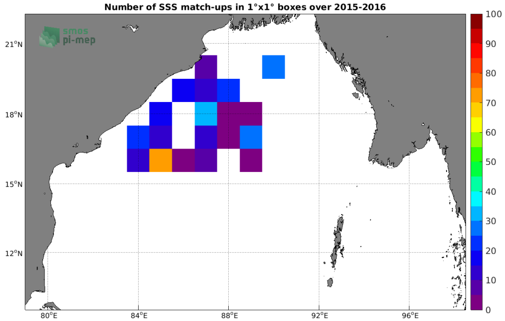
Figure 3: Number of SSS match-ups between Surface drifters SSS and the SMOS L4 v2 Weekly (CATDS-CECOS-IFREMER) SSS product for the Bay of Bengal Pi-MEP region over 1^\circ \times 1^\circ boxes and for the full satellite product period.
