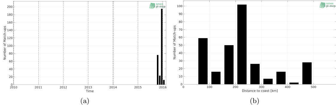
Figure 1: Number of match-ups between Surface drifters and SMOS L4 v2 Weekly (CATDS-CECOS-IFREMER) SSS as a function of time (a) and as function of the distance to coast (b) over the Bay of Bengal Pi-MEP region and for the full satellite product period.
