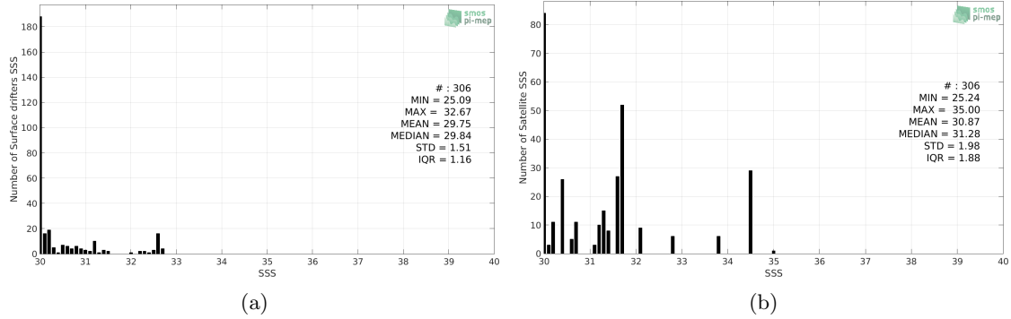
Figure 2: Histograms of SSS from Surface drifters (a) and SMOS-L4-CATDS-CECOS-IFREMER-V2-WEEKLY-0.5DEG (b) considering all match-up pairs per bins of 0.1 over the Bay of Bengal Pi-MEP region and for the full satellite product period.
