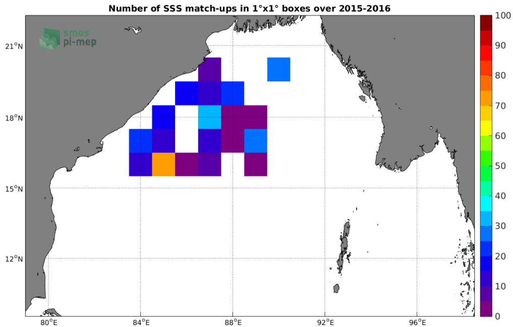
Figure 3: Number of SSS match-ups between Surface drifters SSS and the SMOS-L4-CATDS-CECOS-IFREMER-V2-WEEKLY-0.5DEG SSS product for the Bay of Bengal Pi-MEP region over 1^\circ \times 1^\circ boxes and for the full satellite product period.
