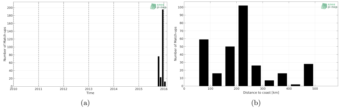
Figure 1: Number of match-ups between Surface drifters and SMOS-L4-CATDS-CECOS-IFREMER-V2-WEEKLY-0.5DEG SSS as a function of time (a) and as function of the distance to coast (b) over the Bay of Bengal Pi-MEP region and for the full satellite product period.
