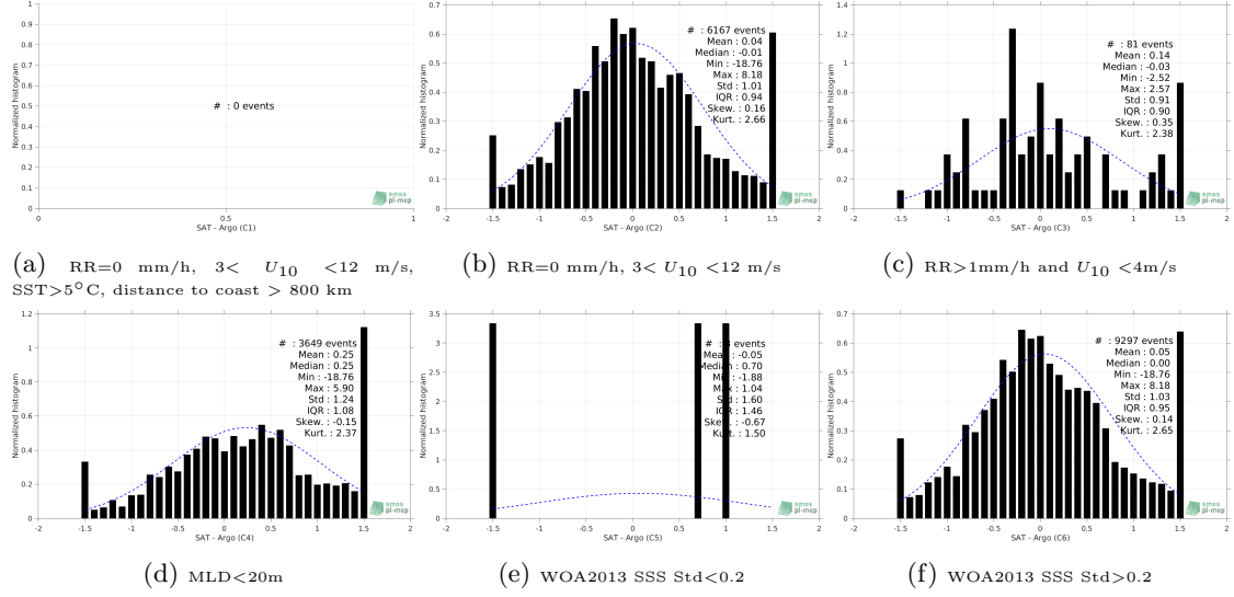
Figure 13: Normalized histogram of \Delta SSS (SMOS-L4-CATDS-CECOS-IFREMER-V2-WEEKLY-0.5DEG - Argo) for 6 different subdatasets corresponding to: RR=0 mm/h, 3 < U_{10} < 12 m/s, SST > 5^\circ\text{C} , distance to coast > 800 km (a), RR=0 mm/h, 3 < U_{10} < 12 m/s (b), RR > 1\text{mm/h} and U_{10} < 4\text{m/s} (c), MLD < 20\text{m} (d), WOA2013 SSS Std < 0.2 (e), WOA2013 SSS Std > 0.2 (f).
