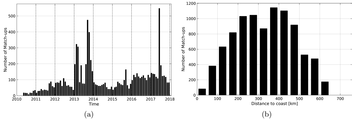
Figure 1: Number of match-ups between Argo and SMOS-L4-CATDS-CECOS-IFREMER-V2-WEEKLY-0.5DEG SSS as a function of time (a) and as function of the distance to coast (b) over the Bay of Bengal Pi-MEP region and for the full satellite product period.
