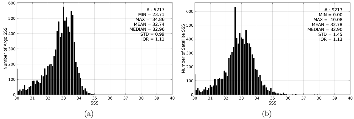
Figure 2: Histograms of SSS from Argo (a) and SMOS-L4-CATDS-CECOS-IFREMER-V2-WEEKLY-0.5DEG (b) considering all match-up pairs per bins of 0.1 over the Bay of Bengal Pi-MEP region and for the full satellite product period.
