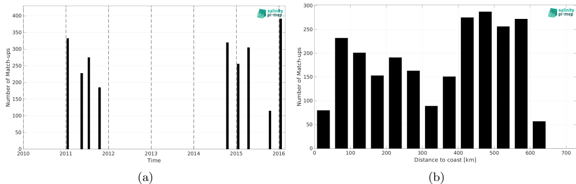
Figure 2: Number of match-ups between TSG (LEGOS-DM) and SMOS SSS L4 v2 - Daily (BEC) SSS as a function of time (a) and as function of the distance to coast (b) over the Bay of Bengal Pi-MEP region and for the full satellite product period.
