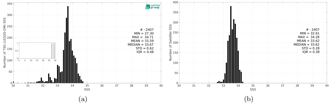
Figure 3: Histograms of SSS from TSG (LEGOS-DM) (a) and SMOS SSS L4 v2 - Daily (BEC) (b) considering all match-up pairs per bins of 0.1 over the Bay of Bengal Pi-MEP region and for the full satellite product period.
