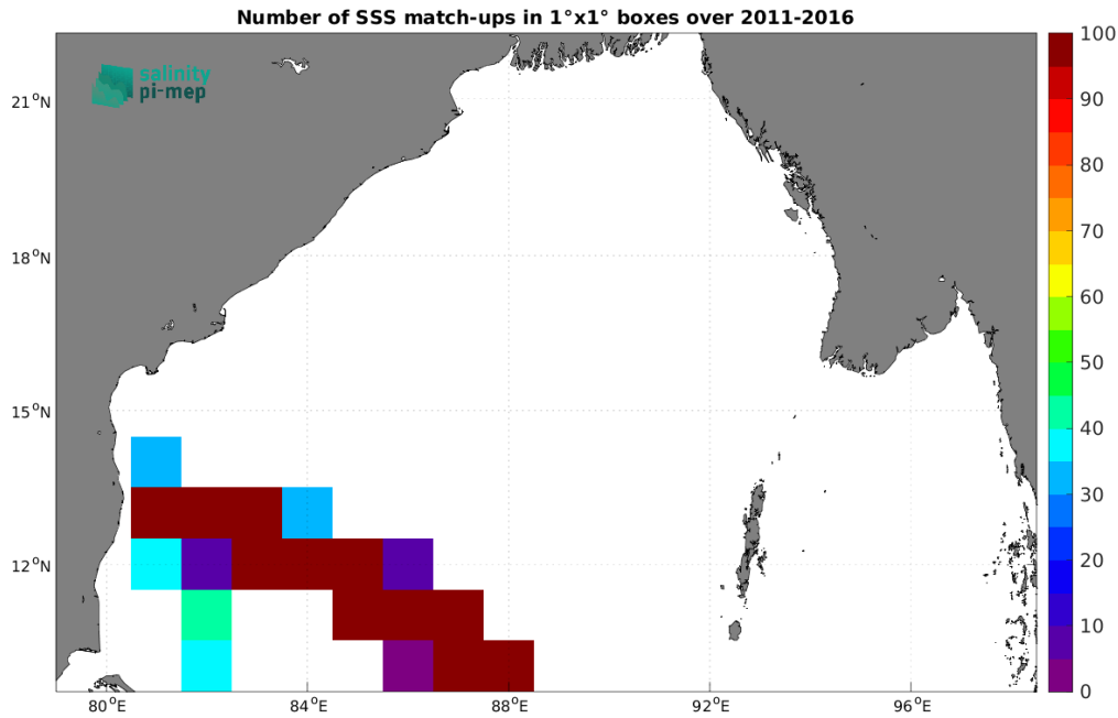
Figure 5: Number of SSS match-ups between TSG (LEGOS-DM) SSS and the SMOS SSS L4 v2 - Daily (BEC) SSS product for the Bay of Bengal Pi-MEP region over 1^\circ \times 1^\circ boxes and for the full satellite product period.
