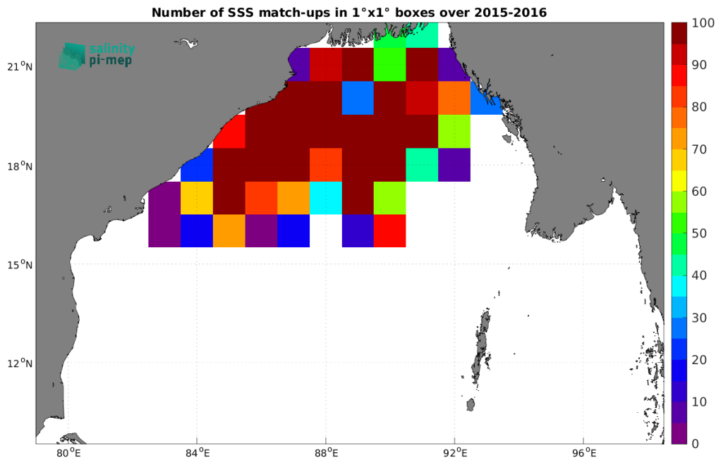
Figure 3: Number of SSS match-ups between Surface drifters SSS and the SMOS SSS L4 v2 - Daily (BEC) SSS product for the Bay of Bengal Pi-MEP region over 1^\circ \times 1^\circ boxes and for the full satellite product period.
