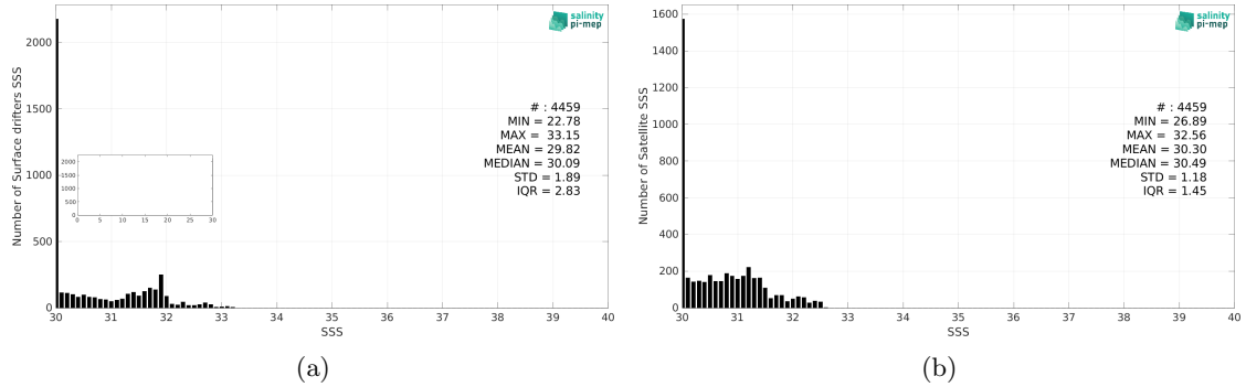
Figure 2: Histograms of SSS from Surface drifters (a) and SMOS SSS L4 v2 - Daily (BEC) (b) considering all match-up pairs per bins of 0.1 over the Bay of Bengal Pi-MEP region and for the full satellite product period.
