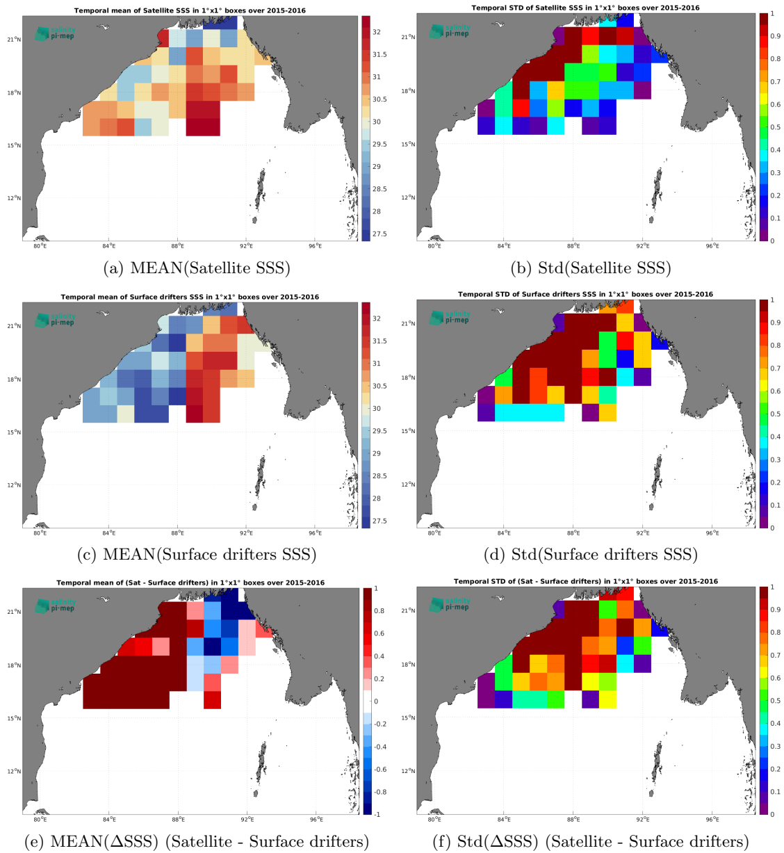
Figure 5: Temporal mean (left) and Std (right) of SSS from SMOS SSS L4 v2 - Daily (BEC) (top), Surface drifters (middle), and of \Delta SSS (Satellite - Surface drifters). Only match-up pairs are used to generate these maps.
