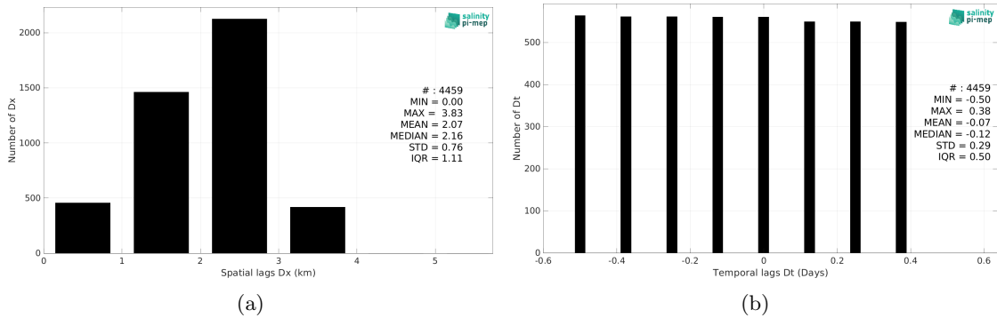
Figure 4: Histograms of the spatial (a) and temporal (b) lags between the location/time of the Surface drifters measurement and the date of the corresponding SMOS SSS L4 v2 - Daily (BEC) SSS pixel.
