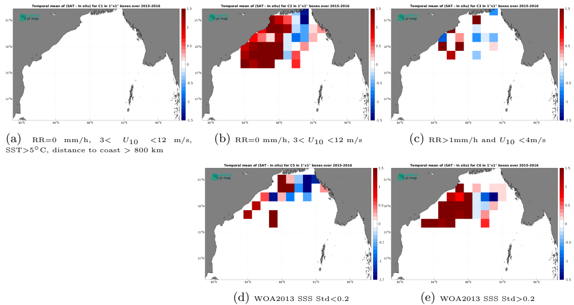
Figure 11: Temporal mean gridded over spatial boxes of size 1^\circ \times 1^\circ of \Delta SSS (SMOS SSS L4 v2 - Daily (BEC) - Surface drifters) for 5 different subdatasets corresponding to:RR=0 mm/h, 3 < U_{10} < 12 m/s, SST > 5^\circ\text{C} , distance to coast > 800 km (a), RR=0 mm/h, 3 < U_{10} < 12 m/s (b), RR > 1 mm/h and U_{10} < 4 m/s (c), WOA2013 SSS Std < 0.2 (d), WOA2013 SSS Std > 0.2 (e).
