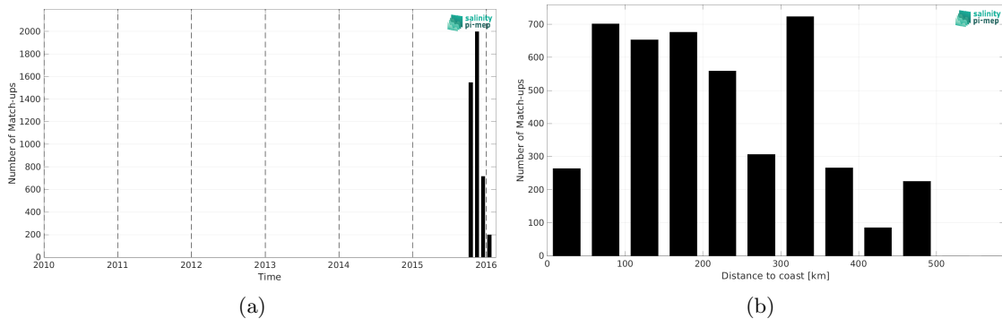
Figure 1: Number of match-ups between Surface drifters and SMOS SSS L4 v2 - Daily (BEC) SSS as a function of time (a) and as function of the distance to coast (b) over the Bay of Bengal Pi-MEP region and for the full satellite product period.
