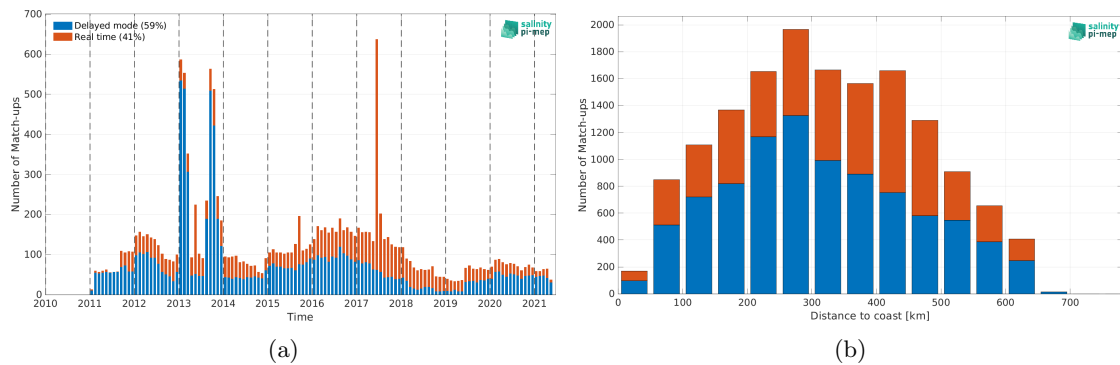
Figure 2: Number of match-ups between Argo and SMOS SSS L4 v2 - Daily (BEC) SSS as a function of time (a) and as function of the distance to coast (b) over the Bay of Bengal Pi-MEP region and for the full satellite product period.
