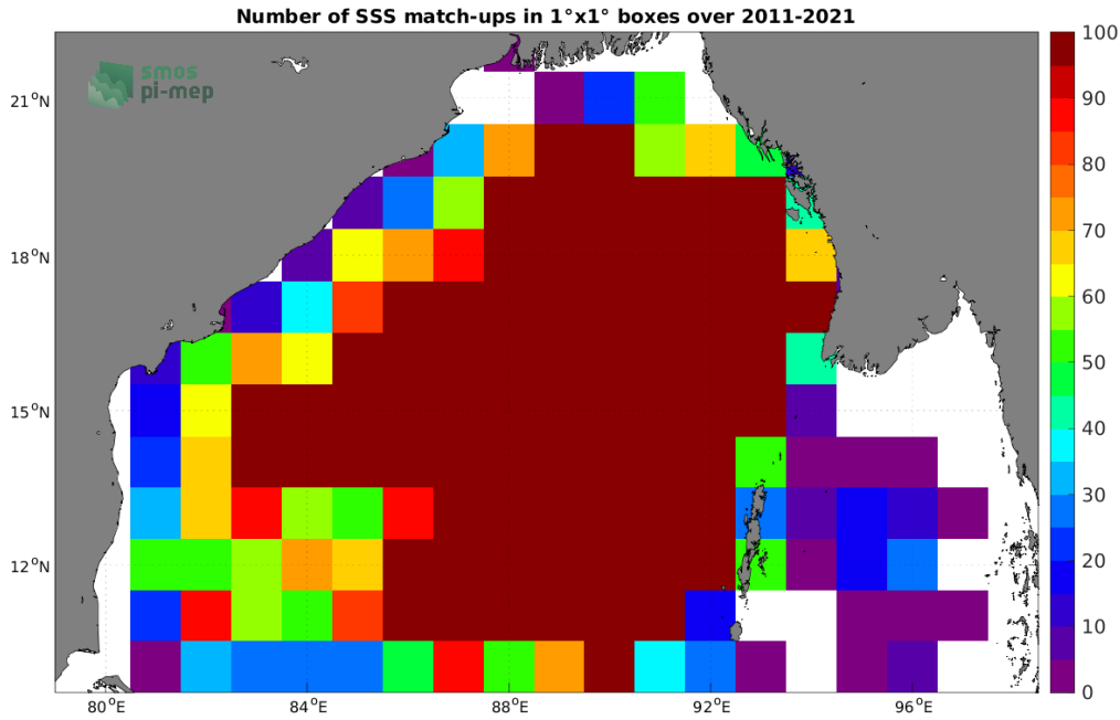
Figure 4: Number of SSS match-ups between Argo SSS and the SMOS SSS L4 v2 - Daily (BEC) SSS product for the Bay of Bengal Pi-MEP region over 1^\circ \times 1^\circ boxes and for the full satellite product period.
