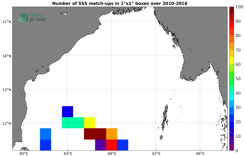
Figure 4: Number of SSS match-ups between TSG (LEGOS-DM) SSS and the SMOS SSS L3 v3 Monthly (ICDC) SSS product for the Bay of Bengal Pi-MEP region over 1^\circ \times 1^\circ boxes and for the full satellite product period.
