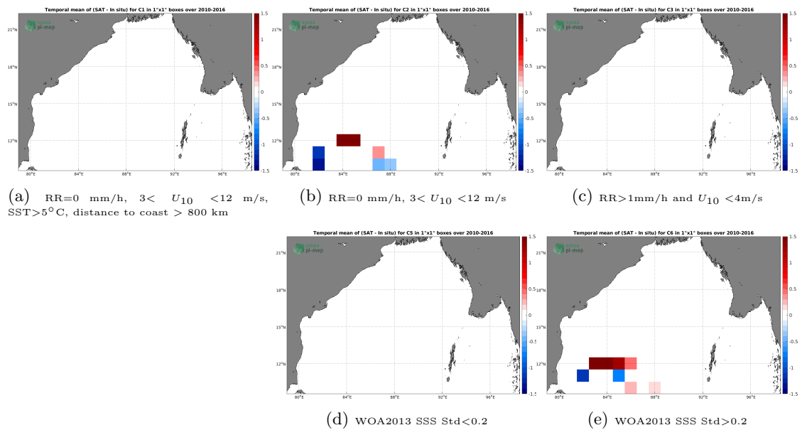
Figure 12: Temporal mean gridded over spatial boxes of size 1°x1° of \Delta SSS (SMOS SSS L3 v3 Monthly (ICDC) - TSG (LEGOS-DM)) for 5 different subdatasets corresponding to: RR=0 mm/h, 3 < U_{10} < 12 m/s, SST > 5°C, distance to coast > 800 km (a), RR=0 mm/h, 3 < U_{10} < 12 m/s (b), RR > 1mm/h and U_{10} < 4 m/s (c), WOA2013 SSS Std < 0.2 (d), WOA2013 SSS Std > 0.2 (e).
