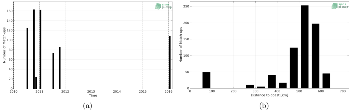
Figure 1: Number of match-ups between TSG (LEGOS-DM) and SMOS SSS L3 v3 Monthly (ICDC) SSS as a function of time (a) and as function of the distance to coast (b) over the Bay of Bengal Pi-MEP region and for the full satellite product period.
