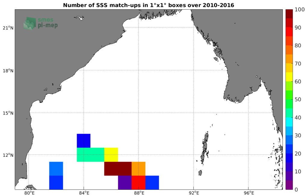
Figure 4: Number of SSS match-ups between TSG (LEGOS-DM) SSS and the SMOS SSS L3 v3 Monthly (ICDC) SSS product for the Bay of Bengal Pi-MEP region over 1°x1° boxes and for the full satellite product period.
