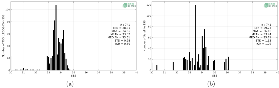
Figure 2: Histograms of SSS from TSG (LEGOS-DM) (a) and SMOS SSS L3 v3 Monthly (ICDC) (b) considering all match-up pairs per bins of 0.1 over the Bay of Bengal Pi-MEP region and for the full satellite product period.
