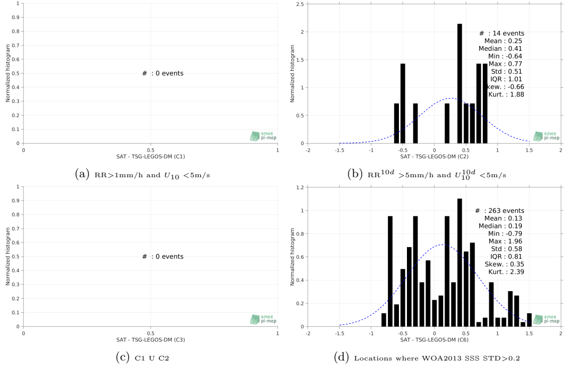
Figure 13: Normalized histogram of \Delta\text{SSS} (SMOS-L3-ICDC-V3-MONTHLY-0.5DEG - TSG-LEGOS-DM) for 6 different subdatasets corresponding to: RR > 1\text{mm/h} and U_{10} < 5\text{m/s} (a), RR^{10d} > 5\text{mm/h} and U_{10}^{10d} < 5\text{m/s} (b), C1 \cup C2 (c), Locations where WOA2013 SSS STD > 0.2 (d).
