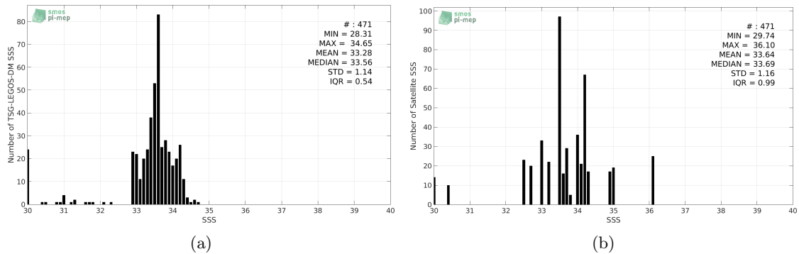
Figure 2: Histograms of SSS from TSG-LEGOS-DM (a) and SMOS-L3-ICDC-V3-MONTHLY-0.5DEG (b) considering all match-up pairs per bins of 0.1 over the Bay of Bengal Pi-MEP region and for the full satellite product period.
