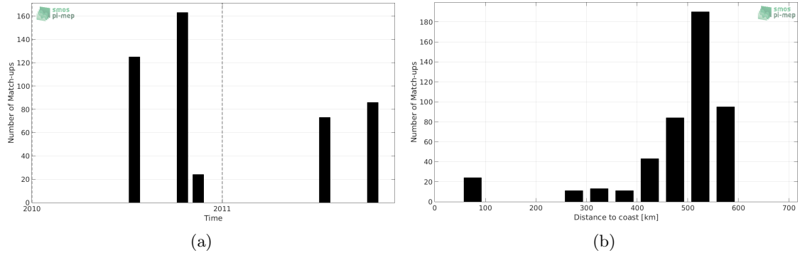
Figure 1: Number of match-ups between TSG-LEGOS-DM and SMOS-L3-ICDC-V3-MONTHLY-0.5DEG SSS as a function of time (a) and as function of the distance to coast (b) over the Bay of Bengal Pi-MEP region and for the full satellite product period.
