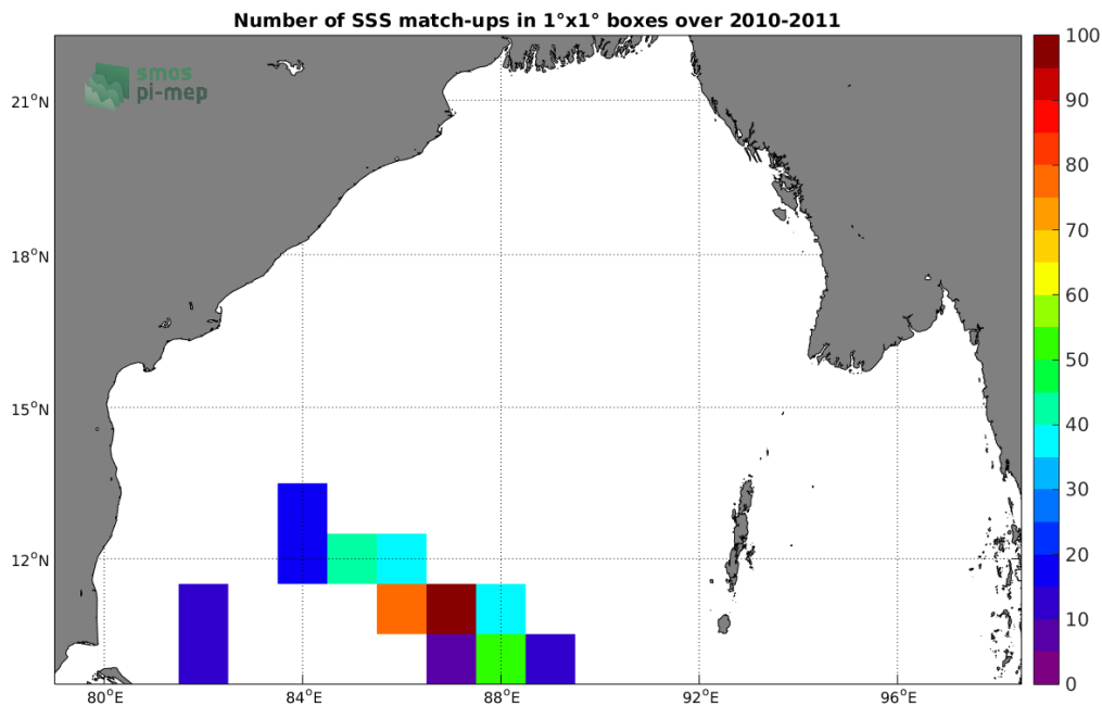
Figure 4: Number of SSS match-ups between TSG-LEGOS-DM SSS and the SMOS-L3-ICDC-V3-MONTHLY-0.5DEG SSS product for the Bay of Bengal Pi-MEP region over 1°x1° boxes and for the full satellite product period.
