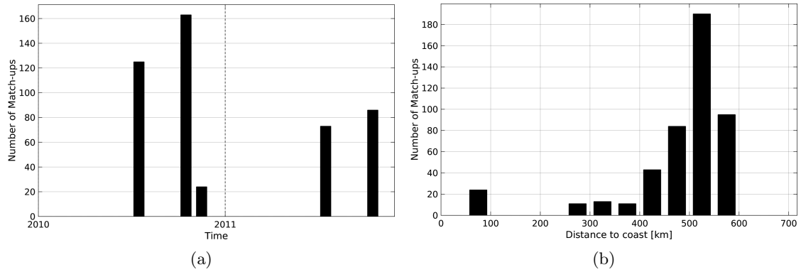
Figure 1: Number of match-ups between TSG-LEGOS-DM and SMOS-L3-ICDC-V3-MONTHLY-0.5DEG SSS as a function of time (a) and as function of the distance to coast (b) over the Bay of Bengal Pi-MEP region and for the full satellite product period.
