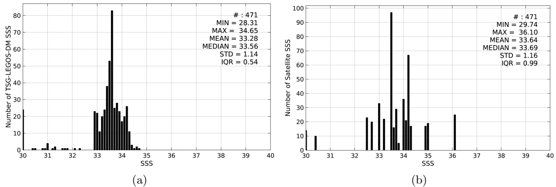
Figure 2: Histograms of SSS from TSG-LEGOS-DM (a) and SMOS-L3-ICDC-V3-MONTHLY-0.5DEG (b) considering all match-up pairs per bins of 0.1 over the Bay of Bengal Pi-MEP region and for the full satellite product period.
