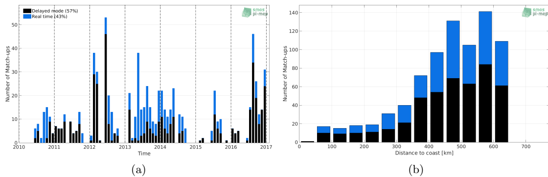
Figure 1: Number of match-ups between Argo and SMOS SSS L3 v3 Monthly (ICDC) SSS as a function of time (a) and as function of the distance to coast (b) over the Bay of Bengal Pi-MEP region and for the full satellite product period.
