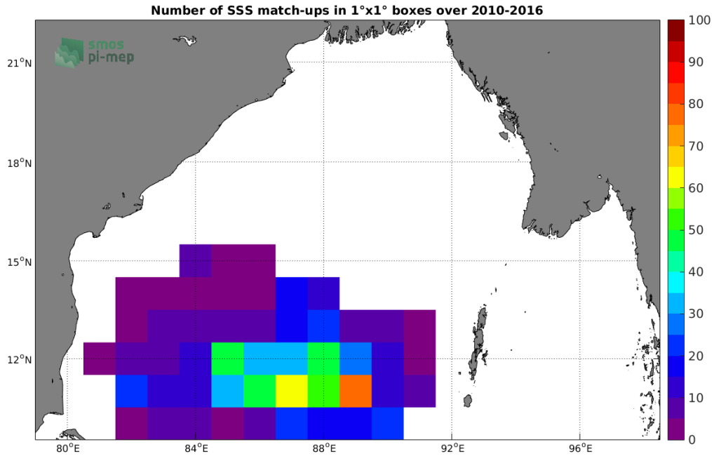
Figure 4: Number of SSS match-ups between Argo SSS and the SMOS SSS L3 v3 Monthly (ICDC) SSS product for the Bay of Bengal Pi-MEP region over 1^\circ \times 1^\circ boxes and for the full satellite product period.
