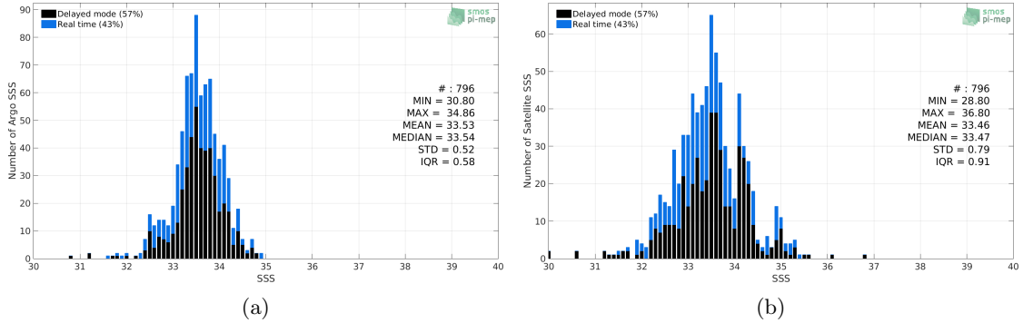
Figure 2: Histograms of SSS from Argo (a) and SMOS SSS L3 v3 Monthly (ICDC) (b) considering all match-up pairs per bins of 0.1 over the Bay of Bengal Pi-MEP region and for the full satellite product period.
