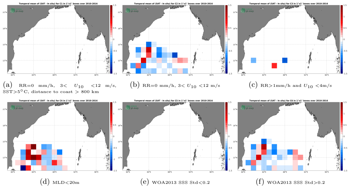
Figure 12: Temporal mean gridded over spatial boxes of size 1°x1° of \Delta SSS (SMOS SSS L3 v3 Monthly (ICDC) - Argo) for 6 different subdatasets corresponding to:RR=0 mm/h, 3 < U_{10} < 12 m/s, SST>5°C, distance to coast > 800 km (a), RR=0 mm/h, 3 < U_{10} < 12 m/s (b), RR>1mm/h and U_{10} < 4 m/s (c),MLD<20m (d),WOA2013 SSS Std<0.2 (e),WOA2013 SSS Std>0.2 (f).
