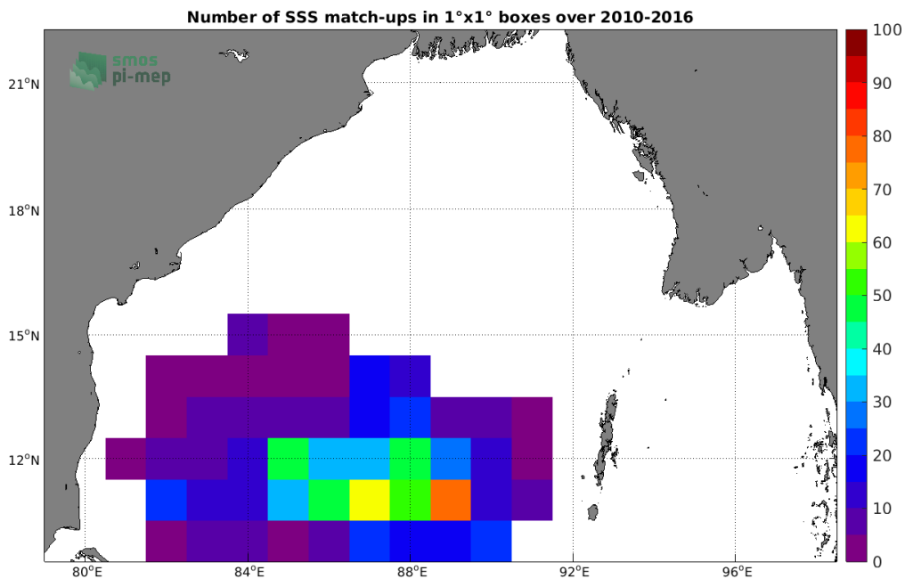
Figure 4: Number of SSS match-ups between Argo SSS and the SMOS SSS L3 v3 Monthly (ICDC) SSS product for the Bay of Bengal Pi-MEP region over 1°x1° boxes and for the full satellite product period.
