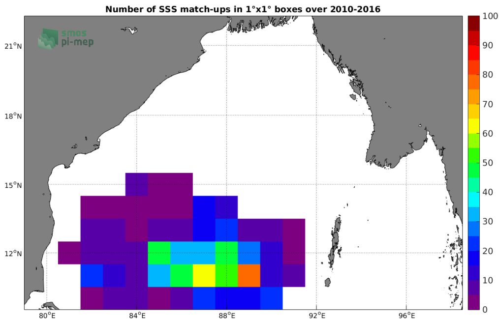
Figure 4: Number of SSS match-ups between Argo SSS and the SMOS-3-ICDC-V3-MONTHLY-0.5DEG SSS product for the Bay of Bengal Pi-MEP region over 1^\circ \times 1^\circ boxes and for the full satellite product period.
