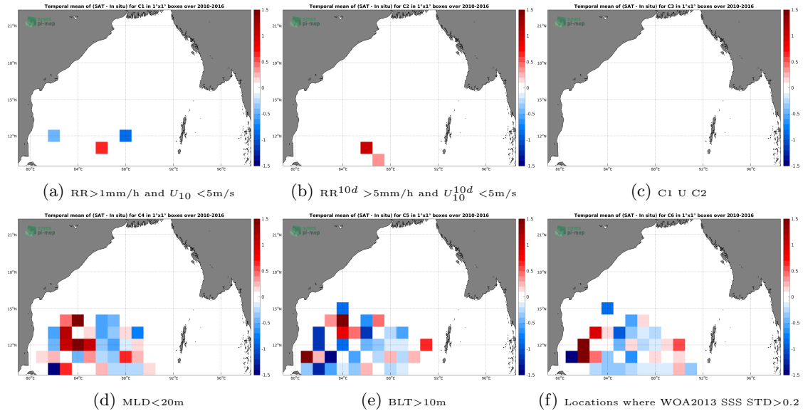
Figure 12: Temporal mean gridded over spatial boxes of size 1^\circ \times 1^\circ of \Delta\text{SSS} (SMOS-L3-ICDC-V3-MONTHLY-0.5DEG - Argo) for 6 different subdatasets corresponding to: RR > 1\text{mm/h} and U_{10} < 5\text{m/s} (a), RR^{10d} > 5\text{mm/h} and U_{10}^{10d} < 5\text{m/s} (b), C1 U C2 (c), MLD < 20\text{m} (d), BLT > 10\text{m} (e), Locations where WOA2013 SSS STD > 0.2 (f).
