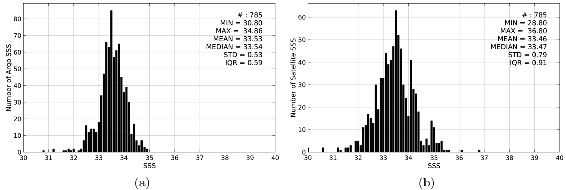
Figure 2: Histograms of SSS from Argo (a) and SMOS-L3-ICDC-V3-MONTHLY-0.5DEG (b) considering all match-up pairs per bins of 0.1 over the Bay of Bengal Pi-MEP region and for the full satellite product period.
