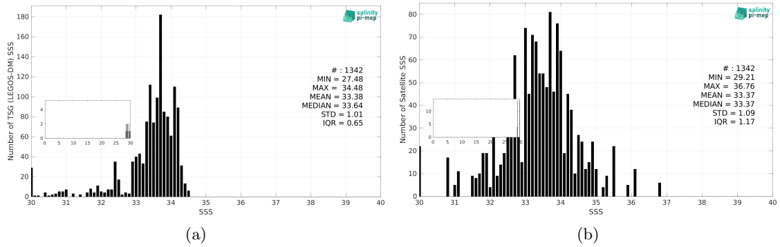
Figure 3: Histograms of SSS from TSG (LEGOS-DM) (a) and SMOS SSS L2Q v331 - With FLAG (CMEMS-CATDS-CPDC) (b) considering all match-up pairs per bins of 0.1 over the Bay of Bengal Pi-MEP region and for the full satellite product period.
