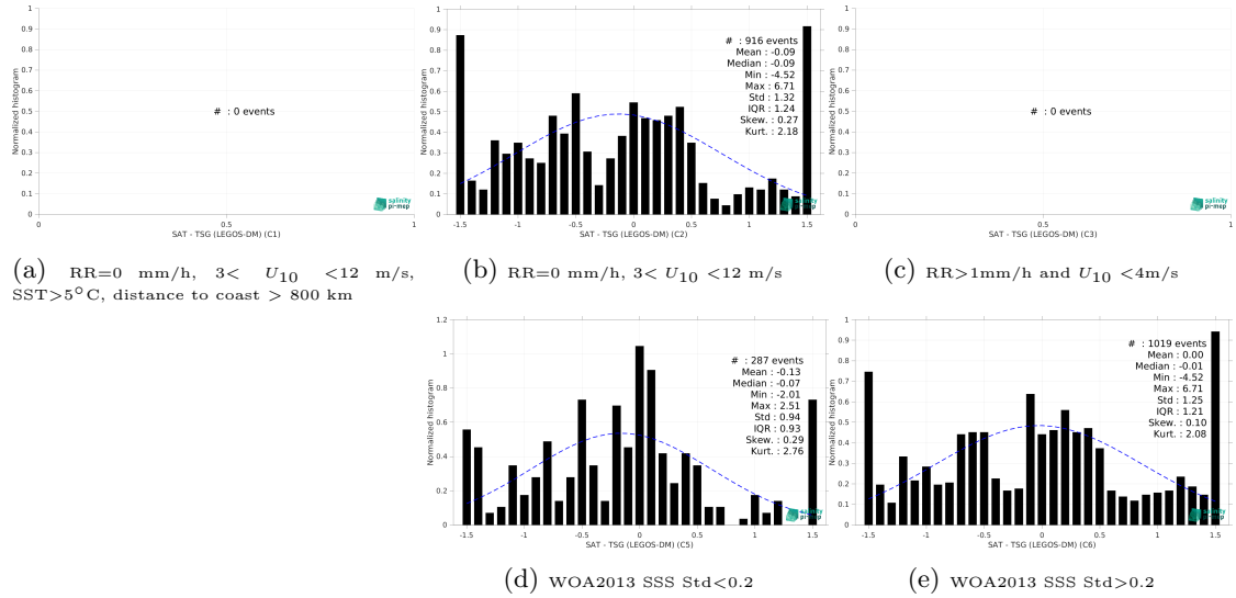
Figure 15: Normalized histogram of \Delta SSS (SMOS SSS L2Q v331 - With FLAG (CMEMS-CATDS-CPDC) - TSG (LEGOS-DM)) for 5 different subdatasets corresponding to: RR=0 mm/h, 3 < U_{10} < 12 m/s, SST > 5°C, distance to coast > 800 km (a), RR=0 mm/h, 3 < U_{10} < 12 m/s (b), RR > 1mm/h and U_{10} < 4 m/s (c), WOA2013 SSS Std < 0.2 (d), WOA2013 SSS Std > 0.2 (e).
