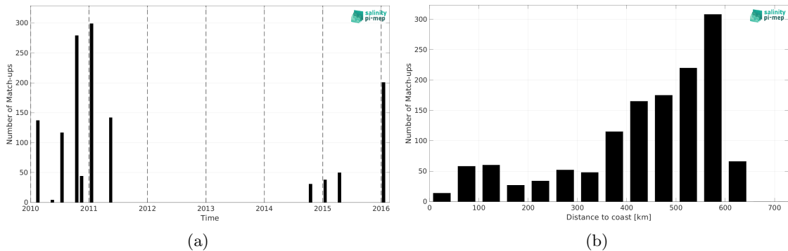
Figure 2: Number of match-ups between TSG (LEGOS-DM) and SMOS SSS L2Q v331 - With FLAG (CMEMS-CATDS-CPDC) SSS as a function of time (a) and as function of the distance to coast (b) over the Bay of Bengal Pi-MEP region and for the full satellite product period.
