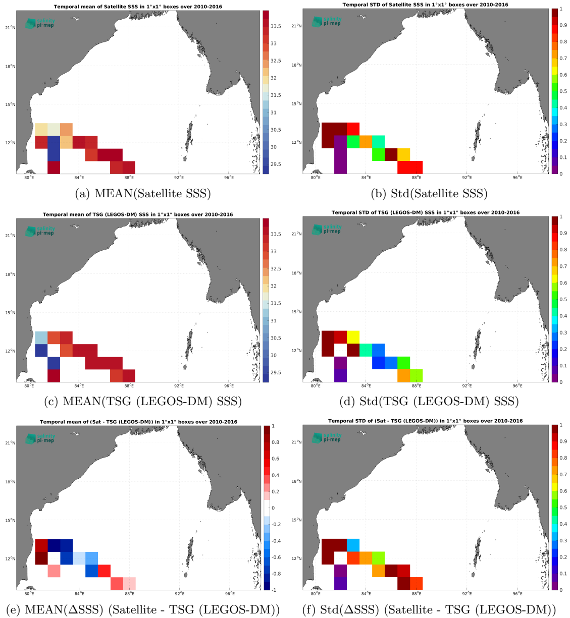
Figure 6: Temporal mean (left) and Std (right) of SSS from SMOS SSS L2Q v331 - With FLAG (CMEMS-CATDS-CPDC) (top), TSG (LEGOS-DM) (middle), and of \Delta SSS (Satellite - TSG (LEGOS-DM)). Only match-up pairs are used to generate these maps.
