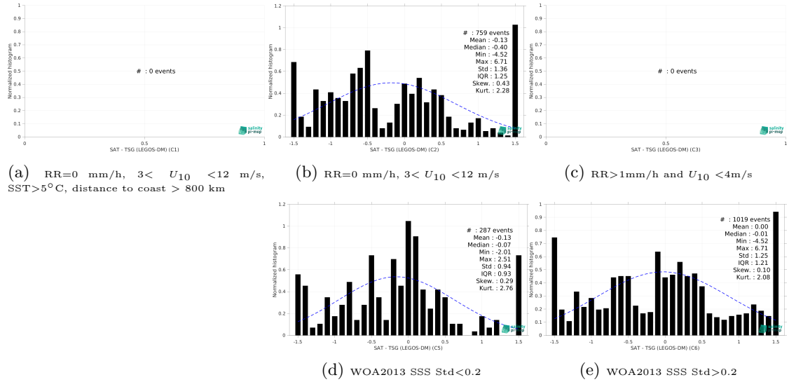
Figure 13: Normalized histogram of \Delta SSS (SMOS SSS L2Q v331 - With FLAG (CMEMS-CATDS-CPDC) - TSG (LEGOS-DM)) for 5 different subdatasets corresponding to: RR=0 mm/h, 3 < U_{10} < 12 m/s, SST > 5°C, distance to coast > 800 km (a), RR=0 mm/h, 3 < U_{10} < 12 m/s (b), RR > 1mm/h and U_{10} < 4 m/s (c), WOA2013 SSS Std < 0.2 (d), WOA2013 SSS Std > 0.2 (e).
