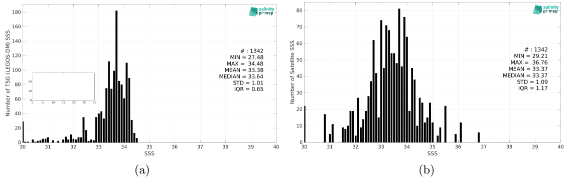
Figure 2: Histograms of SSS from TSG (LEGOS-DM) (a) and SMOS SSS L2Q v331 - With FLAG (CMEMS-CATDS-CPDC) (b) considering all match-up pairs per bins of 0.1 over the Bay of Bengal Pi-MEP region and for the full satellite product period.
