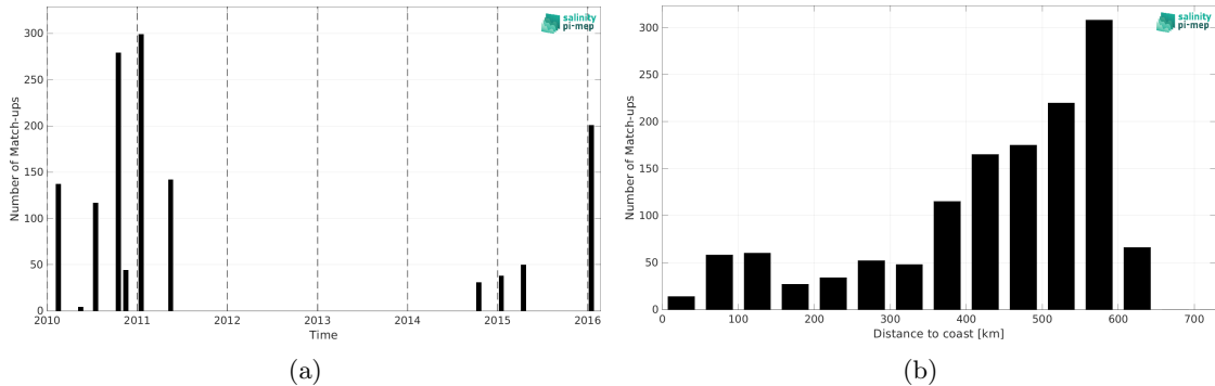
Figure 1: Number of match-ups between TSG (LEGOS-DM) and SMOS SSS L2Q v331 - With FLAG (CMEMS-CATDS-CPDC) SSS as a function of time (a) and as function of the distance to coast (b) over the Bay of Bengal Pi-MEP region and for the full satellite product period.
