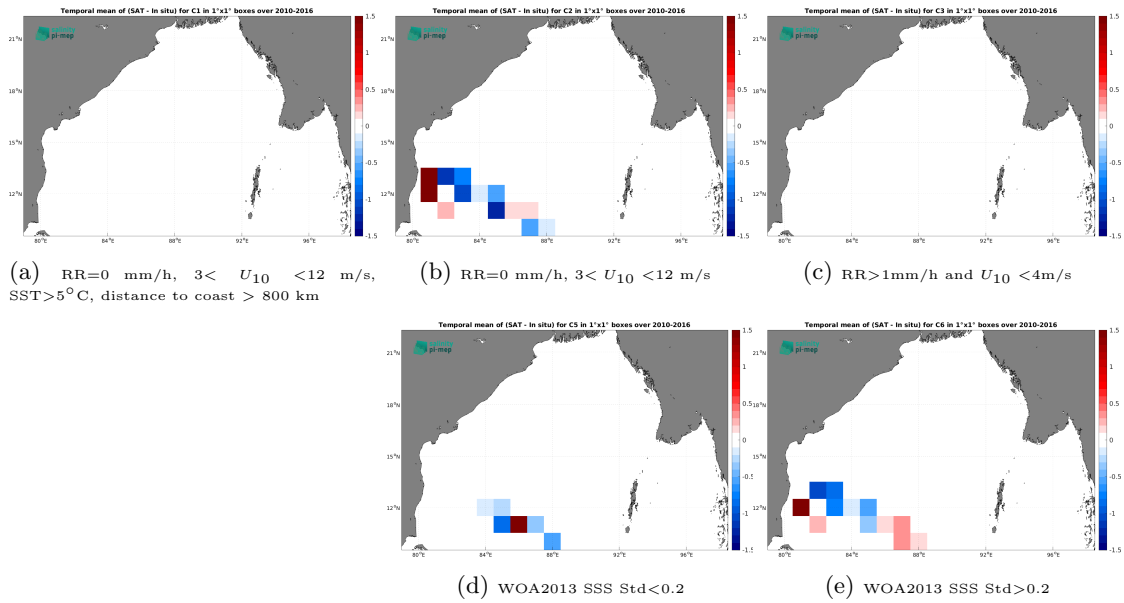
Figure 12: Temporal mean gridded over spatial boxes of size 1^{\circ}\times 1^{\circ} of \Delta\text{SSS} (SMOS SSS L2Q v331 - With FLAG (CMEMS-CATDS-CPDC) - TSG (LEGOS-DM)) for 5 different subdatasets corresponding to:RR=0 mm/h, 3 < U_{10} < 12 m/s, SST > 5^{\circ}\text{C} , distance to coast > 800 km (a), RR=0 mm/h, 3 < U_{10} < 12 m/s (b), RR > 1 mm/h and U_{10} < 4 m/s (c), WOA2013 SSS Std < 0.2 (d), WOA2013 SSS Std > 0.2 (e).
