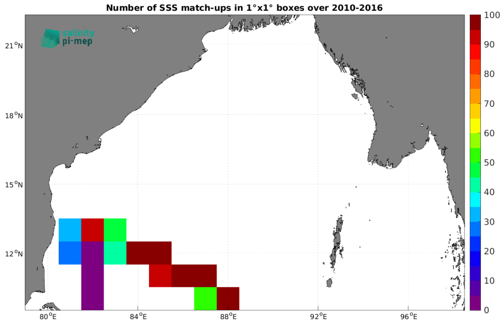
Figure 4: Number of SSS match-ups between TSG (LEGOS-DM) SSS and the SMOS SSS L2Q v331 - With FLAG (CMEMS-CATDS-CPDC) SSS product for the Bay of Bengal Pi-MEP region over 1^\circ \times 1^\circ boxes and for the full satellite product period.
