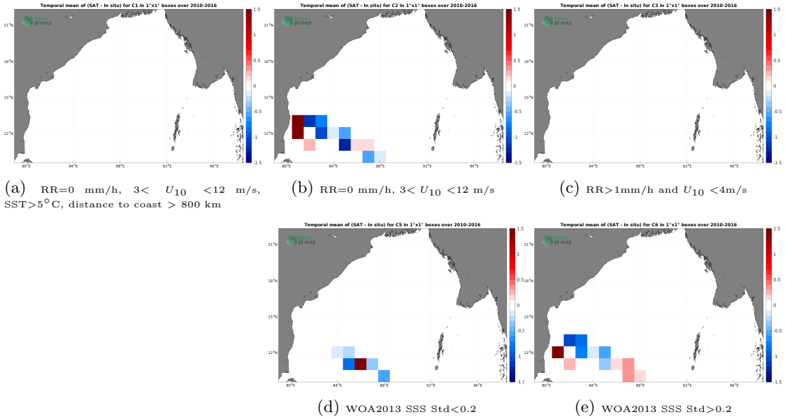
Figure 12: Temporal mean gridded over spatial boxes of size 1^{\circ}\times 1^{\circ} of \Delta\text{SSS} (SMOS SSS L2Q v331 - With FLAG (CMEMS-CATDS-CPDC) - TSG (LEGOS-DM)) for 5 different subdatasets corresponding to:RR=0 mm/h, 3 < U_{10} < 12 m/s, SST > 5^{\circ}\text{C} , distance to coast > 800 km (a), RR=0 mm/h, 3 < U_{10} < 12 m/s (b), RR > 1 mm/h and U_{10} < 4 m/s (c), WOA2013 SSS Std < 0.2 (d), WOA2013 SSS Std > 0.2 (e).
