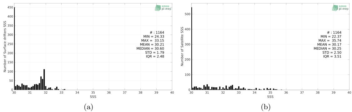
Figure 2: Histograms of SSS from Surface drifters (a) and SMOS SSS L2Q v331 - With FLAG (CMEMS-CATDS-CPDC) (b) considering all match-up pairs per bins of 0.1 over the Bay of Bengal Pi-MEP region and for the full satellite product period.
