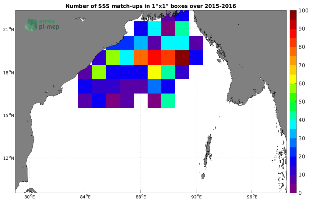
Figure 3: Number of SSS match-ups between Surface drifters SSS and the SMOS SSS L2Q v331 - With FLAG (CMEMS-CATDS-CPDC) SSS product for the Bay of Bengal Pi-MEP region over 1^\circ \times 1^\circ boxes and for the full satellite product period.
