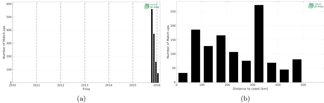
Figure 1: Number of match-ups between Surface drifters and SMOS SSS L2Q v331 - With FLAG (CMEMS-CATDS-CPDC) SSS as a function of time (a) and as function of the distance to coast (b) over the Bay of Bengal Pi-MEP region and for the full satellite product period.
