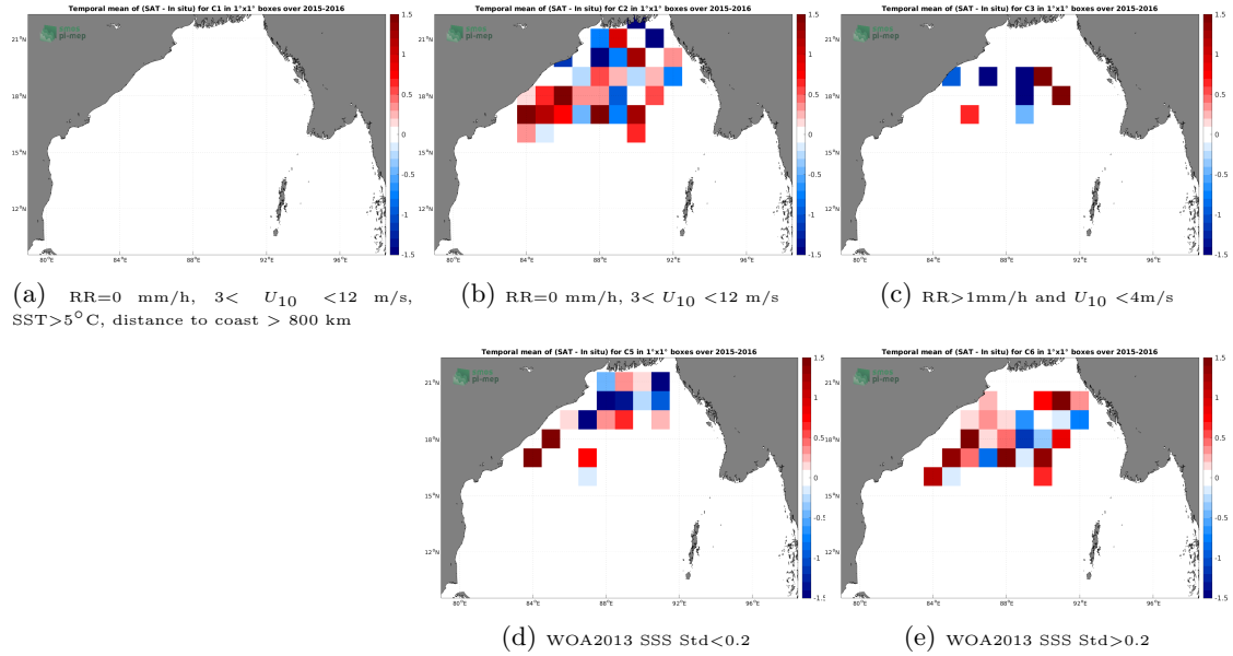
Figure 11: Temporal mean gridded over spatial boxes of size 1^{\circ}\times 1^{\circ} of \Delta\text{SSS} (SMOS SSS L2Q v331 - With FLAG (CMEMS-CATDS-CPDC) - Surface drifters) for 5 different subdatasets corresponding to:RR=0 mm/h, 3 < U_{10} < 12 m/s, SST > 5^{\circ}\text{C} , distance to coast > 800 km (a), RR=0 mm/h, 3 < U_{10} < 12 m/s (b), RR > 1 mm/h and U_{10} < 4 m/s (c), WOA2013 SSS Std < 0.2 (d), WOA2013 SSS Std > 0.2 (e).
