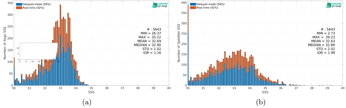
Figure 2: Histograms of SSS from Argo (a) and SMOS SSS L2Q v331 - With FLAG (CMEMS-CATDS-CPDC) (b) considering all match-up pairs per bins of 0.1 over the Bay of Bengal Pi-MEP region and for the full satellite product period.
