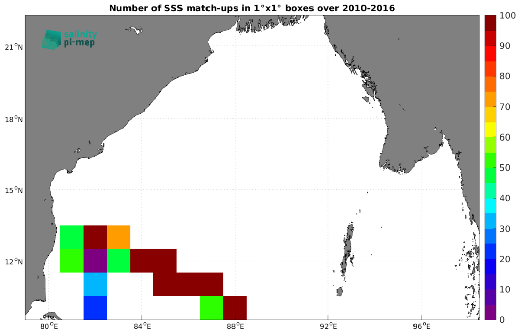
Figure 5: Number of SSS match-ups between TSG (LEGOS-DM) SSS and the SMOS SSS L2Q v331 - No FLAG (CMEMS-CATDS-CPDC) SSS product for the Bay of Bengal Pi-MEP region over 1^\circ \times 1^\circ boxes and for the full satellite product period.
