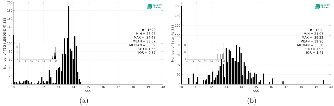
Figure 3: Histograms of SSS from TSG (LEGOS-DM) (a) and SMOS SSS L2Q v331 - No FLAG (CMEMS-CATDS-CPDC) (b) considering all match-up pairs per bins of 0.1 over the Bay of Bengal Pi-MEP region and for the full satellite product period.
