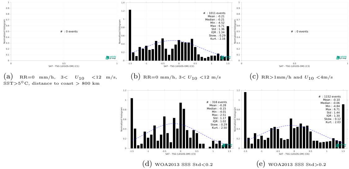
Figure 15: Normalized histogram of \Delta SSS (SMOS SSS L2Q v331 - No FLAG (CMEMS-CATDS-CPDC) - TSG (LEGOS-DM)) for 5 different subdatasets corresponding to: RR=0 mm/h, 3 < U_{10} < 12 m/s, SST > 5°C, distance to coast > 800 km (a), RR=0 mm/h, 3 < U_{10} < 12 m/s (b), RR > 1mm/h and U_{10} < 4 m/s (c), WOA2013 SSS Std < 0.2 (d), WOA2013 SSS Std > 0.2 (e).
