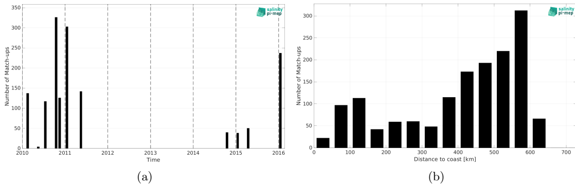
Figure 2: Number of match-ups between TSG (LEGOS-DM) and SMOS SSS L2Q v331 - No FLAG (CMEMS-CATDS-CPDC) SSS as a function of time (a) and as function of the distance to coast (b) over the Bay of Bengal Pi-MEP region and for the full satellite product period.
