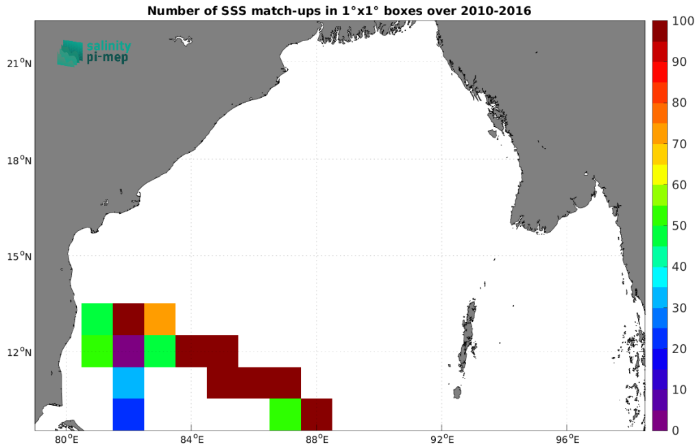
Figure 4: Number of SSS match-ups between TSG (LEGOS-DM) SSS and the SMOS SSS L2Q v331 - No FLAG (CMEMS-CATDS-CPDC) SSS product for the Bay of Bengal Pi-MEP region over 1^\circ \times 1^\circ boxes and for the full satellite product period.
