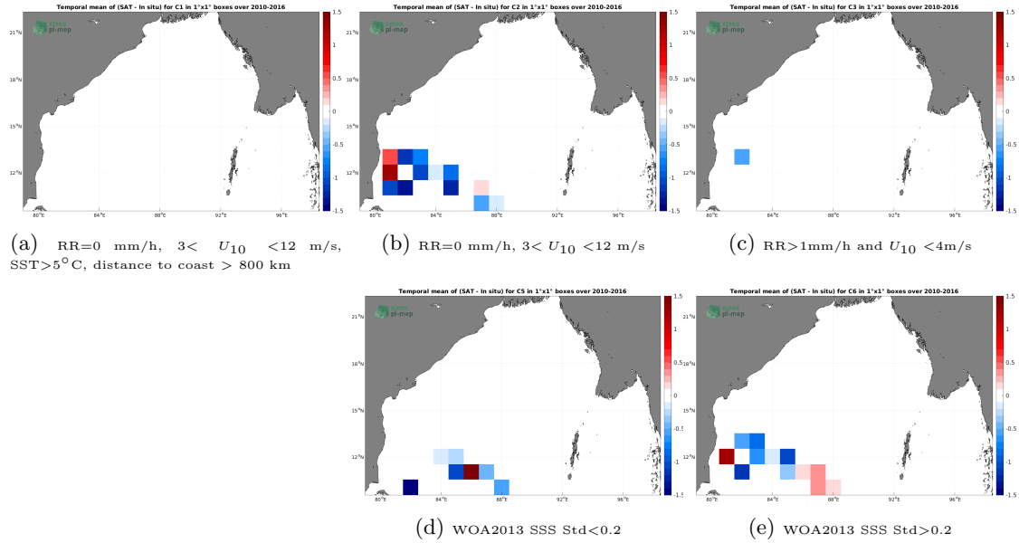
Figure 12: Temporal mean gridded over spatial boxes of size 1^{\circ}\times 1^{\circ} of \Delta\text{SSS} (SMOS SSS L2Q v331 - No FLAG (CMEMS-CATDS-CPDC) - TSG (LEGOS-DM)) for 5 different subdatasets corresponding to:RR=0 mm/h, 3 < U_{10} < 12 m/s, SST > 5^{\circ}\text{C} , distance to coast > 800 km (a), RR=0 mm/h, 3 < U_{10} < 12 m/s (b), RR > 1 mm/h and U_{10} < 4 m/s (c), WOA2013 SSS Std < 0.2 (d), WOA2013 SSS Std > 0.2 (e).
