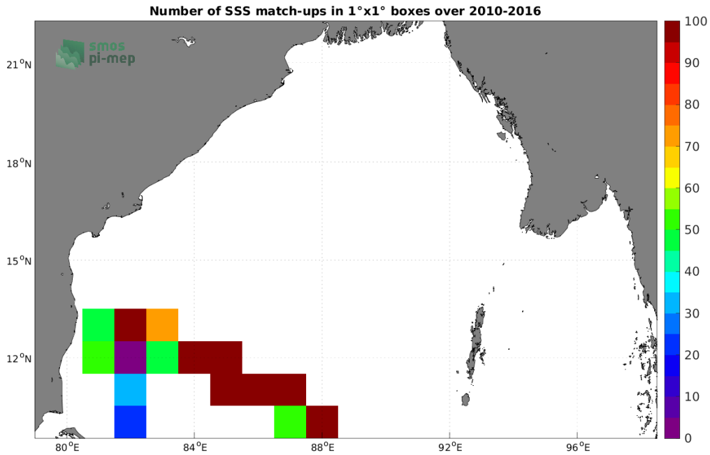
Figure 4: Number of SSS match-ups between TSG (LEGOS-DM) SSS and the SMOS SSS L2Q v331 - No FLAG (CMEMS-CATDS-CPDC) SSS product for the Bay of Bengal Pi-MEP region over 1°×1° boxes and for the full satellite product period.
