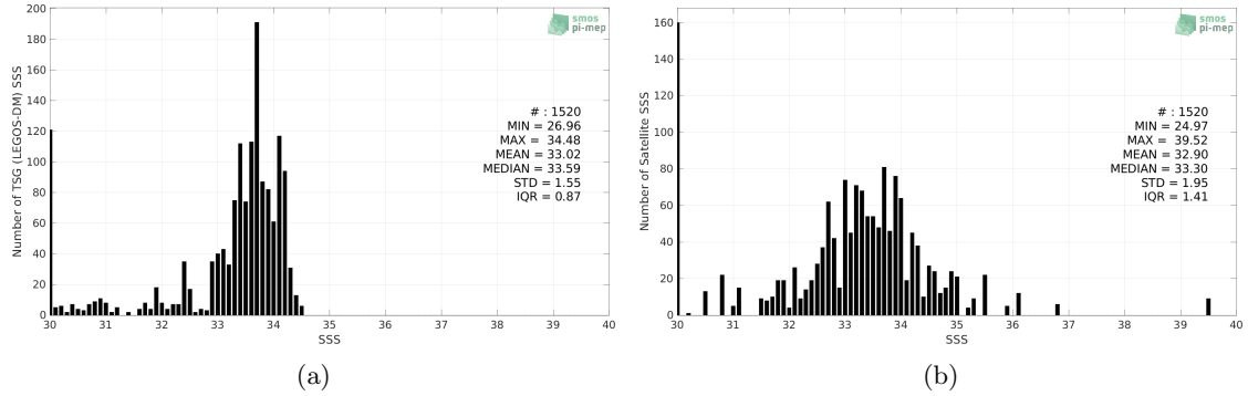
Figure 2: Histograms of SSS from TSG (LEGOS-DM) (a) and SMOS SSS L2Q v331 - No FLAG (CMEMS-CATDS-CPDC) (b) considering all match-up pairs per bins of 0.1 over the Bay of Bengal Pi-MEP region and for the full satellite product period.
