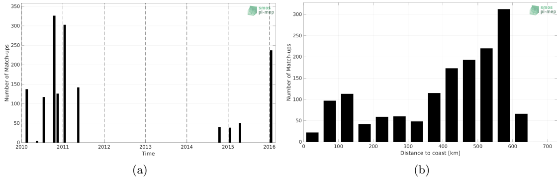
Figure 1: Number of match-ups between TSG (LEGOS-DM) and SMOS SSS L2Q v331 - No FLAG (CMEMS-CATDS-CPDC) SSS as a function of time (a) and as function of the distance to coast (b) over the Bay of Bengal Pi-MEP region and for the full satellite product period.
