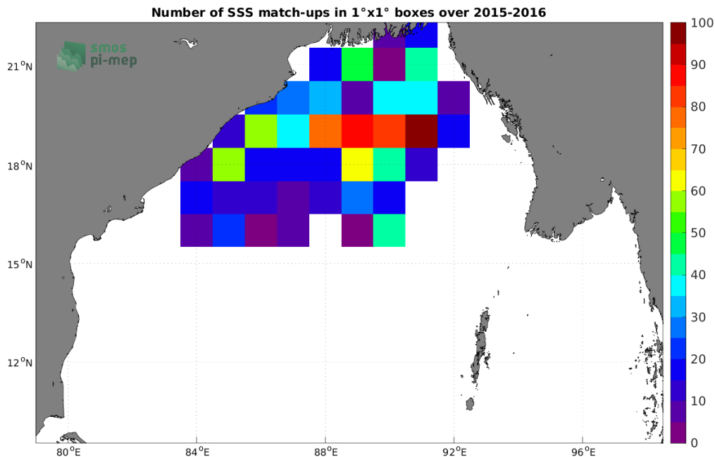
Figure 3: Number of SSS match-ups between Surface drifters SSS and the SMOS SSS L2Q v331 - No FLAG (CMEMS-CATDS-CPDC) SSS product for the Bay of Bengal Pi-MEP region over 1^\circ \times 1^\circ boxes and for the full satellite product period.
