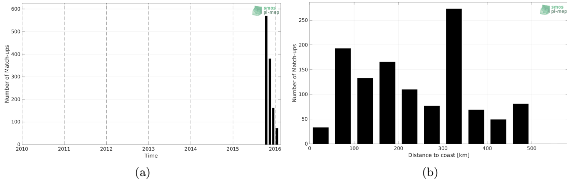
Figure 1: Number of match-ups between Surface drifters and SMOS SSS L2Q v331 - No FLAG (CMEMS-CATDS-CPDC) SSS as a function of time (a) and as function of the distance to coast (b) over the Bay of Bengal Pi-MEP region and for the full satellite product period.
