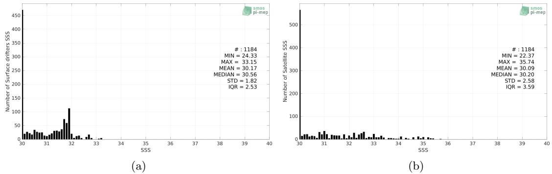
Figure 2: Histograms of SSS from Surface drifters (a) and SMOS SSS L2Q v331 - No FLAG (CMEMS-CATDS-CPDC) (b) considering all match-up pairs per bins of 0.1 over the Bay of Bengal Pi-MEP region and for the full satellite product period.
