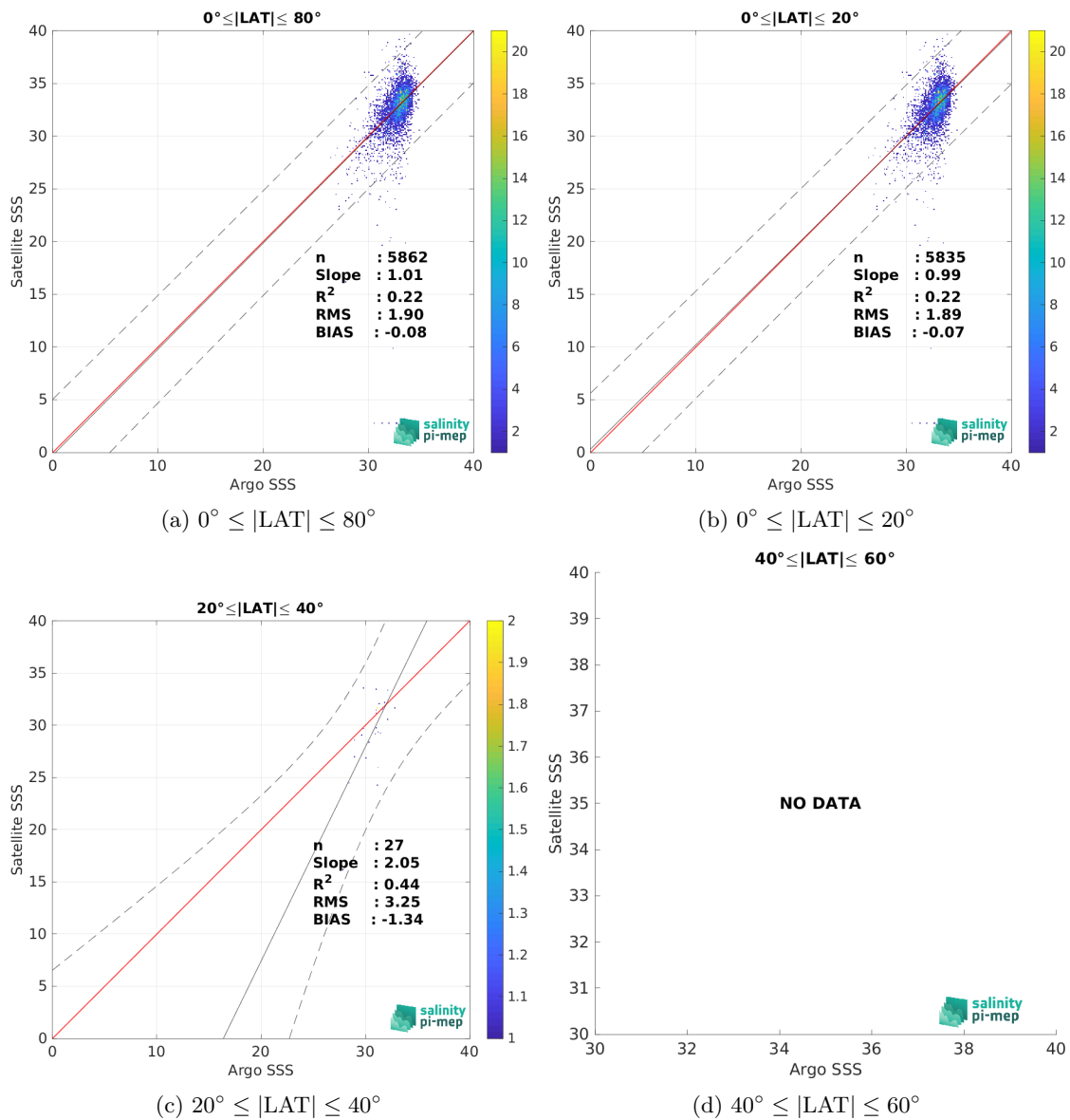
Figure 9: Contour maps of the concentration of SMOS SSS L2Q v331 - No FLAG (CMEMS-CATDS-CPDC) SSS ( y -axis) versus Argo SSS ( x -axis) at match-up pairs for different latitude bands. For each plot, the red line shows x=y . The black thin and dashed lines indicate a linear fit through the data cloud and the \pm 95\% confidence levels, respectively. The number match-up pairs n , the slope and R^2 coefficient of the linear fit, the root mean square (RMS) and the mean bias between satellite and in situ data are indicated for each latitude band in each plots.
