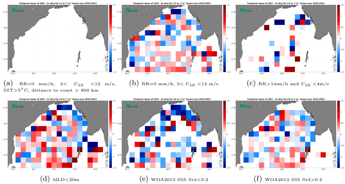
Figure 12: Temporal mean gridded over spatial boxes of size 1^\circ \times 1^\circ of \Delta SSS (SMOS SSS L2Q v331 - No FLAG (CMEMS-CATDS-CPDC) - Argo) for 6 different subdatasets corresponding to:RR=0 mm/h, 3 < U_{10} < 12 m/s, SST >5^\circ C, distance to coast > 800 km (a), RR=0 mm/h, 3 < U_{10} < 12 m/s (b), RR >1 mm/h and U_{10} < 4 m/s (c),MLD <20 m (d),WOA2013 SSS Std <0.2 (e),WOA2013 SSS Std >0.2 (f).
