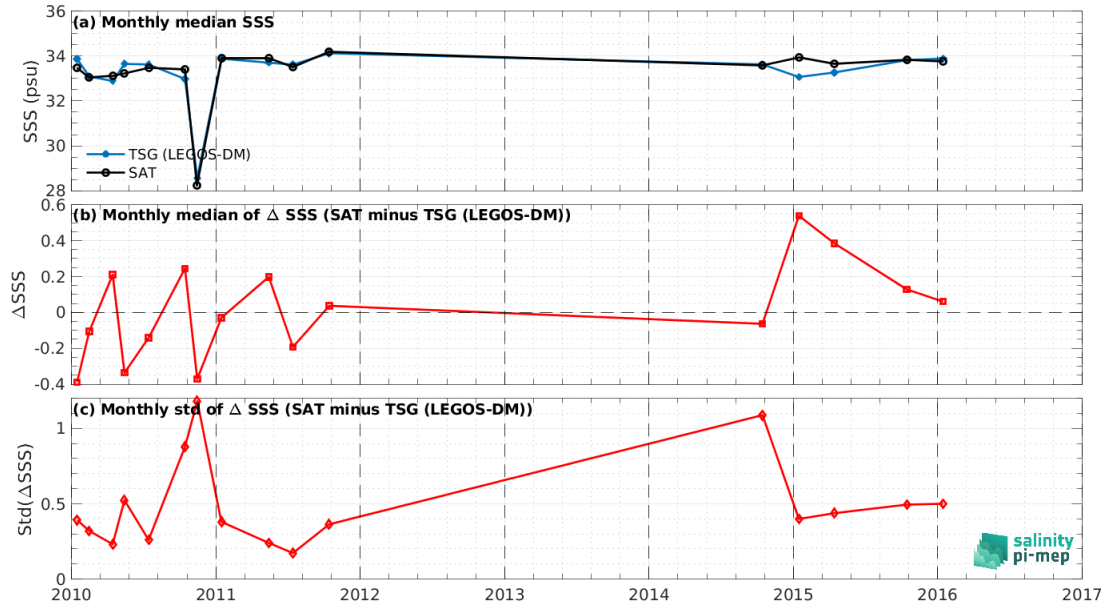
Figure 8: Time series of the monthly median SSS (top), median of \Delta\text{SSS} (Satellite - TSG (LEGOS-DM)) and Std of \Delta\text{SSS} (Satellite - TSG (LEGOS-DM)) over the Bay of Bengal Pi-MEP region considering all match-ups collected by the Pi-MEP.
