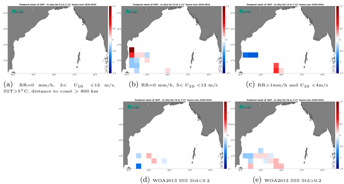
Figure 14: Temporal mean gridded over spatial boxes of size 1^\circ \times 1^\circ of \Delta\text{SSS} (SMOS SSS L3 v9 - 9 Days (CATDS-CEC-LOCEAN) - TSG (LEGOS-DM)) for 5 different subdatasets corresponding to:RR=0 mm/h, 3 < U_{10} < 12 m/s, SST >5^\circ\text{C} , distance to coast > 800 km (a), RR=0 mm/h, 3 < U_{10} < 12 m/s (b), RR >1 mm/h and U_{10} < 4 m/s (c), WOA2013 SSS Std <0.2 (d), WOA2013 SSS Std >0.2 (e).
