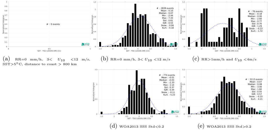
Figure 15: Normalized histogram of \Delta SSS (SMOS SSS L3 v9 - 9 Days (CATDS-CEC-LOCEAN) - TSG (LEGOS-DM)) for 5 different subdatasets corresponding to: RR=0 mm/h, 3 < U_{10} < 12 m/s, SST > 5°C, distance to coast > 800 km (a), RR=0 mm/h, 3 < U_{10} < 12 m/s (b), RR > 1mm/h and U_{10} < 4 m/s (c), WOA2013 SSS Std < 0.2 (d), WOA2013 SSS Std > 0.2 (e).
