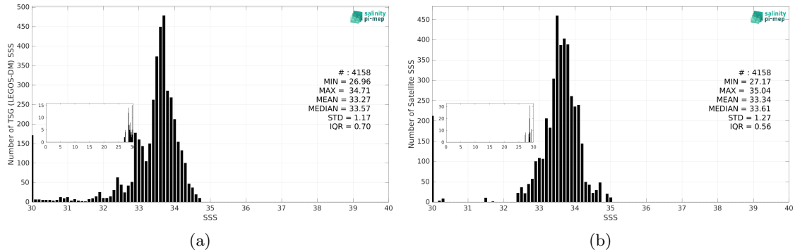
Figure 3: Histograms of SSS from TSG (LEGOS-DM) (a) and SMOS SSS L3 v9 - 9 Days (CATDS-CEC-LOCEAN) (b) considering all match-up pairs per bins of 0.1 over the Bay of Bengal Pi-MEP region and for the full satellite product period.
