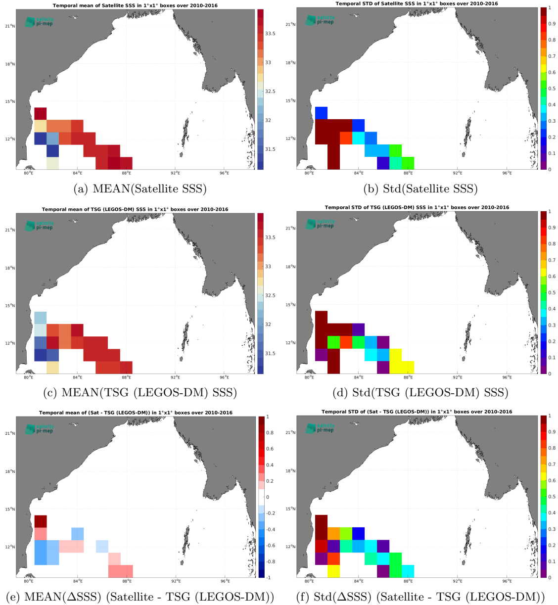
Figure 7: Temporal mean (left) and Std (right) of SSS from SMOS SSS L3 v9 - 9 Days (CATDS-CEC-LOCEAN) (top), TSG (LEGOS-DM) (middle), and of \Delta SSS (Satellite - TSG (LEGOS-DM)). Only match-up pairs are used to generate these maps.
