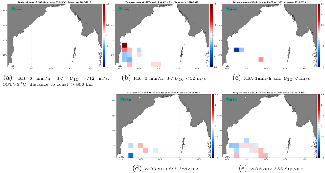
Figure 12: Temporal mean gridded over spatial boxes of size 1^{\circ}\times 1^{\circ} of \Delta\text{SSS} (SMOS SSS L3 v9 - 9 Days (CATDS-CEC-LOCEAN) - TSG (LEGOS-DM)) for 5 different subdatasets corresponding to:RR=0 mm/h, 3 < U_{10} < 12 m/s, SST > 5^{\circ}\text{C} , distance to coast > 800 km (a), RR=0 mm/h, 3 < U_{10} < 12 m/s (b), RR > 1 mm/h and U_{10} < 4 m/s (c), WOA2013 SSS Std < 0.2 (d), WOA2013 SSS Std > 0.2 (e).
