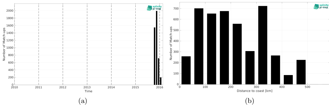
Figure 1: Number of match-ups between Surface drifters and SMOS SSS L3 v9 - 9 Days (CATDS-CEC-LOCEAN) SSS as a function of time (a) and as function of the distance to coast (b) over the Bay of Bengal Pi-MEP region and for the full satellite product period.
