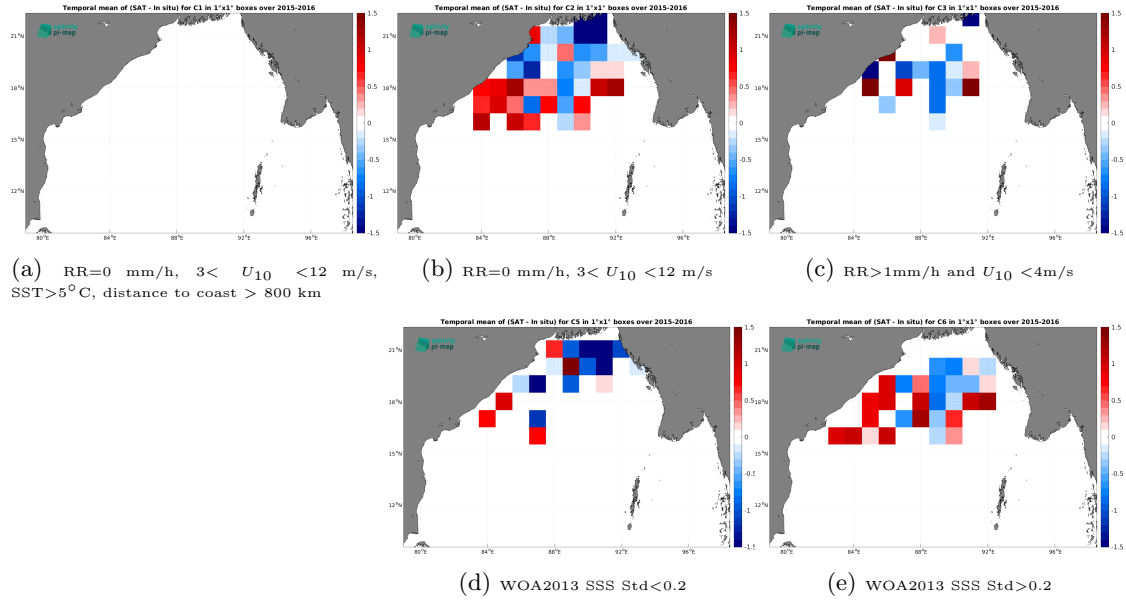
Figure 11: Temporal mean gridded over spatial boxes of size 1^{\circ}\times 1^{\circ} of \Delta\text{SSS} (SMOS SSS L3 v9 - 9 Days (CATDS-CEC-LOCEAN) - Surface drifters) for 5 different subdatasets corresponding to:RR=0 mm/h, 3 < U_{10} < 12 m/s, SST > 5^{\circ}\text{C} , distance to coast > 800 km (a), RR=0 mm/h, 3 < U_{10} < 12 m/s (b), RR > 1 mm/h and U_{10} < 4 m/s (c), WOA2013 SSS Std < 0.2 (d), WOA2013 SSS Std > 0.2 (e).
