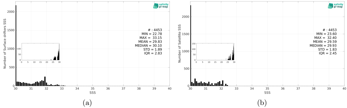
Figure 2: Histograms of SSS from Surface drifters (a) and SMOS SSS L3 v9 - 9 Days (CATDS-CEC-LOCEAN) (b) considering all match-up pairs per bins of 0.1 over the Bay of Bengal Pi-MEP region and for the full satellite product period.
