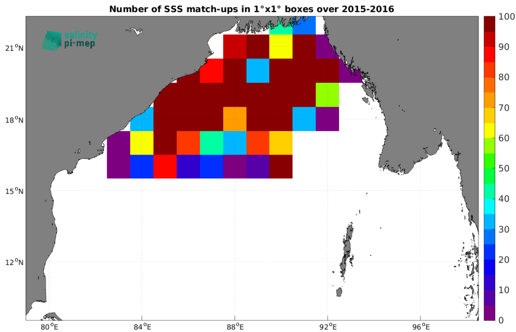
Figure 3: Number of SSS match-ups between Surface drifters SSS and the SMOS SSS L3 v9 - 9 Days (CATDS-CEC-LOCEAN) SSS product for the Bay of Bengal Pi-MEP region over 1^\circ \times 1^\circ boxes and for the full satellite product period.
