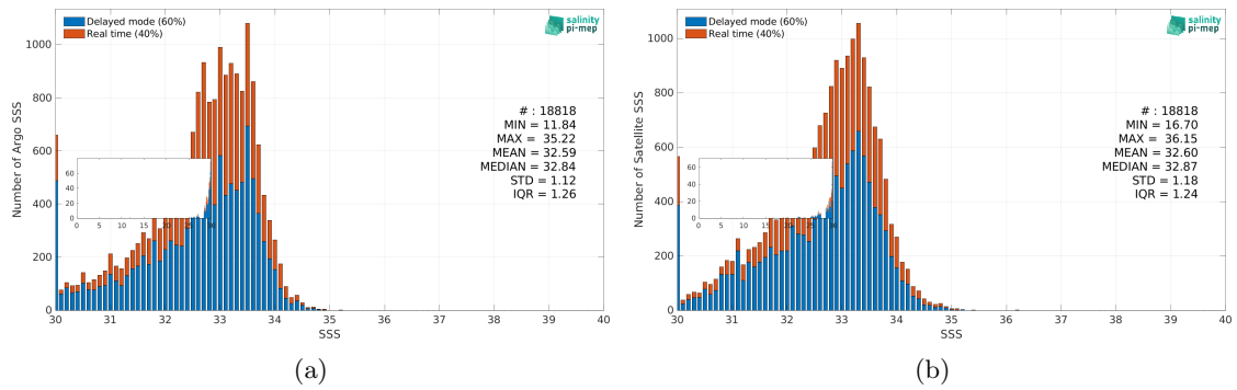
Figure 2: Histograms of SSS from Argo (a) and SMOS SSS L3 v9 - 9 Days (CATDS-CEC-LOCEAN) (b) considering all match-up pairs per bins of 0.1 over the Bay of Bengal Pi-MEP region and for the full satellite product period.
