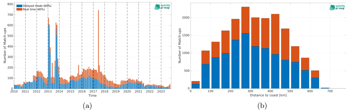
Figure 1: Number of match-ups between Argo and SMOS SSS L3 v9 - 9 Days (CATDS-CEC-LOCEAN) SSS as a function of time (a) and as function of the distance to coast (b) over the Bay of Bengal Pi-MEP region and for the full satellite product period.
