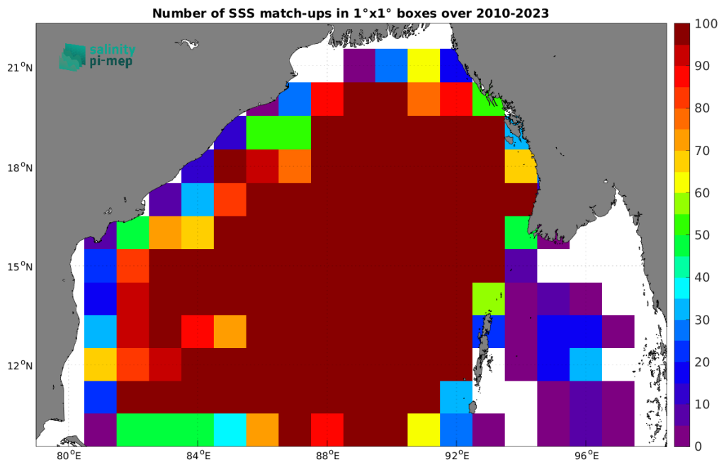
Figure 4: Number of SSS match-ups between Argo SSS and the SMOS SSS L3 v9 - 9 Days (CATDS-CEC-LOCEAN) SSS product for the Bay of Bengal Pi-MEP region over 1^\circ \times 1^\circ boxes and for the full satellite product period.
