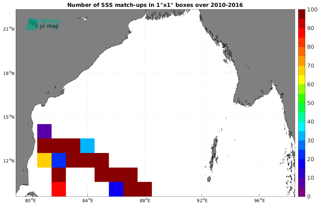
Figure 5: Number of SSS match-ups between TSG (LEGOS-DM) SSS and the SMOS SSS L3 v9 - 18 Days (CATDS-CEC-LOCEAN) SSS product for the Bay of Bengal Pi-MEP region over 1^{\circ} \times 1^{\circ} boxes and for the full satellite product period.
