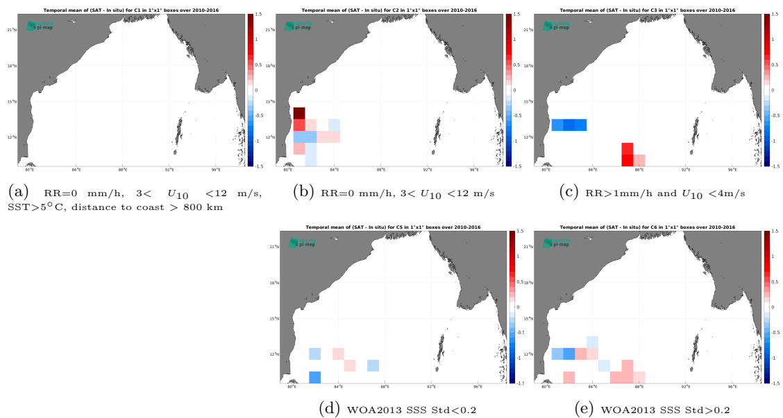
Figure 14: Temporal mean gridded over spatial boxes of size 1^\circ \times 1^\circ of \Delta\text{SSS} (SMOS SSS L3 v9 - 18 Days (CATDS-CEC-LOCEAN) - TSG (LEGOS-DM)) for 5 different subdatasets corresponding to:RR=0 mm/h, 3 < U_{10} < 12 m/s, SST >5^\circ\text{C} , distance to coast > 800 km (a), RR=0 mm/h, 3 < U_{10} < 12 m/s (b), RR >1 mm/h and U_{10} < 4 m/s (c), WOA2013 SSS Std <0.2 (d), WOA2013 SSS Std >0.2 (e).
