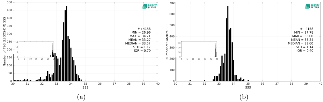
Figure 3: Histograms of SSS from TSG (LEGOS-DM) (a) and SMOS SSS L3 v9 - 18 Days (CATDS-CEC-LOCEAN) (b) considering all match-up pairs per bins of 0.1 over the Bay of Bengal Pi-MEP region and for the full satellite product period.
