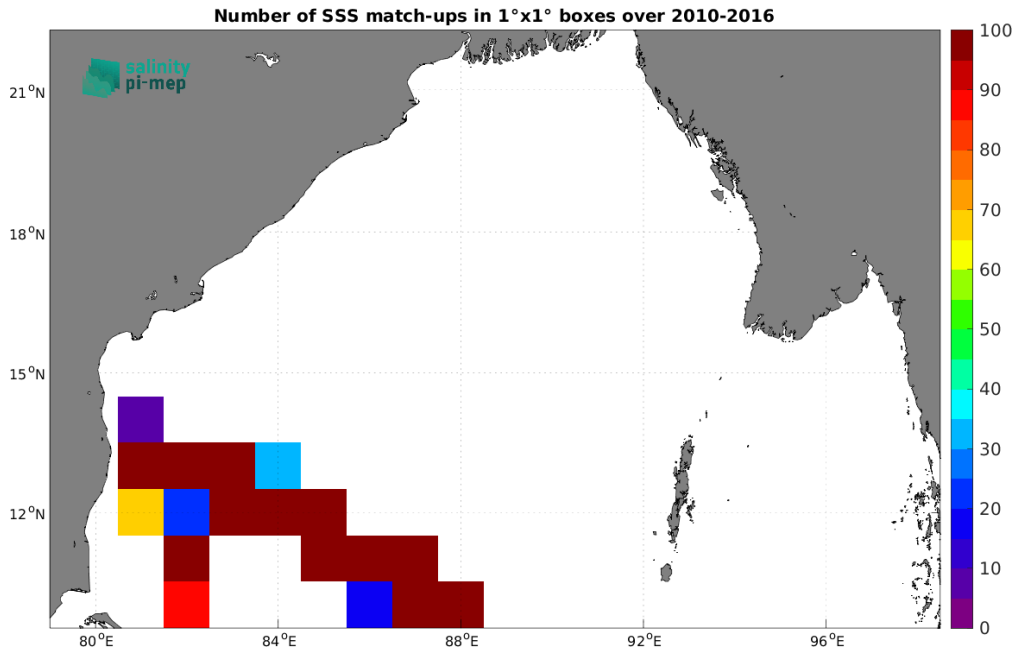
Figure 5: Number of SSS match-ups between TSG (LEGOS-DM) SSS and the SMOS SSS L3 v9 - 18 Days (CATDS-CEC-LOCEAN) SSS product for the Bay of Bengal Pi-MEP region over 1^\circ \times 1^\circ boxes and for the full satellite product period.
