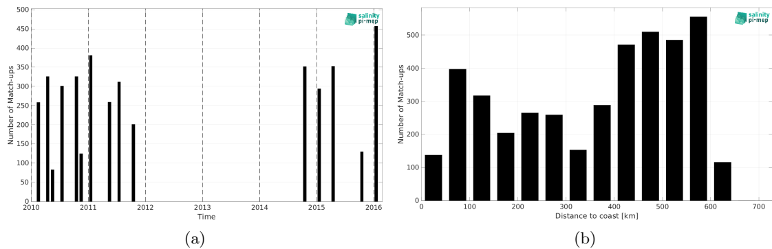
Figure 2: Number of match-ups between TSG (LEGOS-DM) and SMOS SSS L3 v9 - 18 Days (CATDS-CEC-LOCEAN) SSS as a function of time (a) and as function of the distance to coast (b) over the Bay of Bengal Pi-MEP region and for the full satellite product period.
