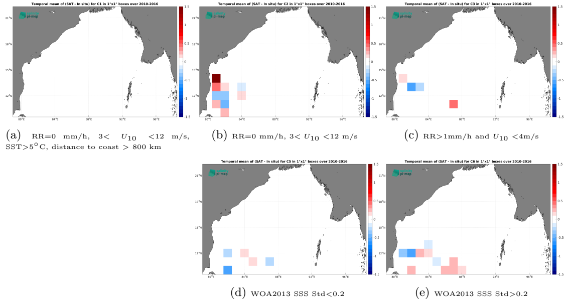
Figure 12: Temporal mean gridded over spatial boxes of size 1^{\circ}\times 1^{\circ} of \Delta\text{SSS} (SMOS SSS L3 v9 - 18 Days (CATDS-CEC-LOCEAN) - TSG (LEGOS-DM)) for 5 different subdatasets corresponding to:RR=0 mm/h, 3 < U_{10} < 12 m/s, SST >5^{\circ}\text{C} , distance to coast > 800 km (a), RR=0 mm/h, 3 < U_{10} < 12 m/s (b), RR >1 mm/h and U_{10} < 4 m/s (c), WOA2013 SSS Std <0.2 (d), WOA2013 SSS Std >0.2 (e).
