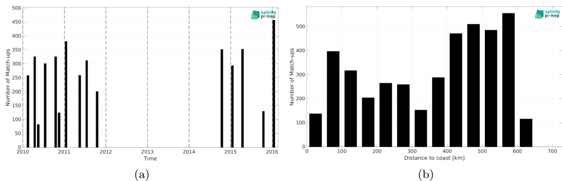
Figure 1: Number of match-ups between TSG (LEGOS-DM) and SMOS SSS L3 v9 - 18 Days (CATDS-CEC-LOCEAN) SSS as a function of time (a) and as function of the distance to coast (b) over the Bay of Bengal Pi-MEP region and for the full satellite product period.
