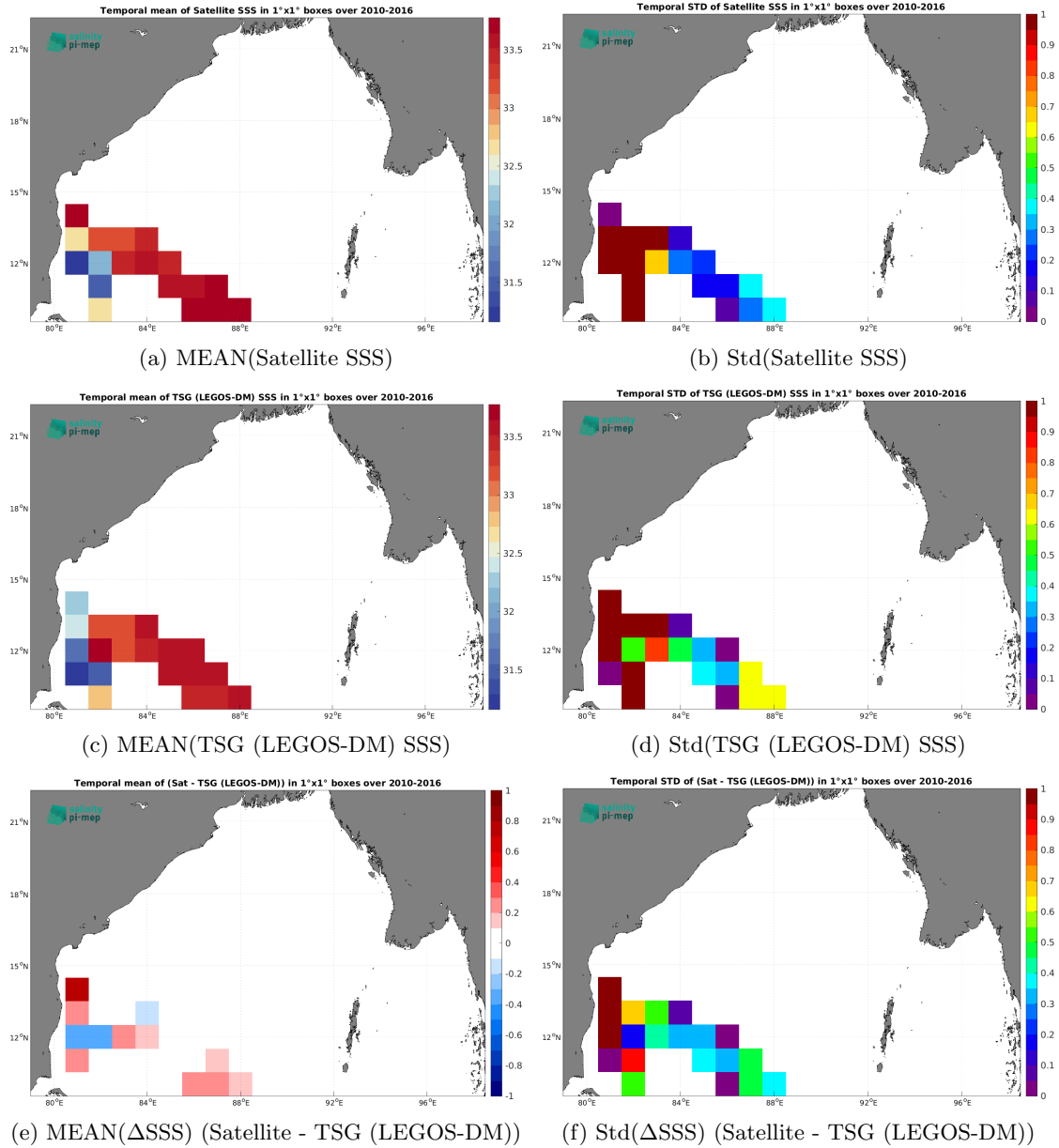
Figure 6: Temporal mean (left) and Std (right) of SSS from SMOS SSS L3 v9 - 18 Days (CATDS-CEC-LOCEAN) (top), TSG (LEGOS-DM) (middle), and of \Delta SSS (Satellite - TSG (LEGOS-DM)). Only match-up pairs are used to generate these maps.
