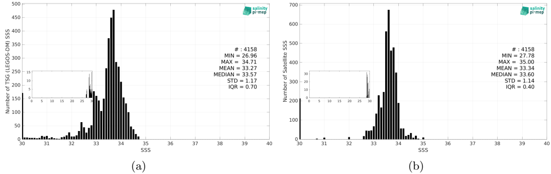
Figure 2: Histograms of SSS from TSG (LEGOS-DM) (a) and SMOS SSS L3 v9 - 18 Days (CATDS-CEC-LOCEAN) (b) considering all match-up pairs per bins of 0.1 over the Bay of Bengal Pi-MEP region and for the full satellite product period.
