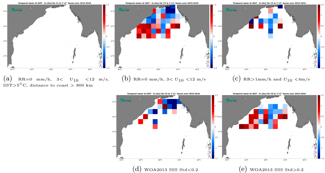
Figure 11: Temporal mean gridded over spatial boxes of size 1^{\circ}\times 1^{\circ} of \Delta\text{SSS} (SMOS SSS L3 v9 - 18 Days (CATDS-CEC-LOCEAN) - Surface drifters) for 5 different subdatasets corresponding to:RR=0 mm/h, 3 < U_{10} < 12 m/s, SST > 5^{\circ}\text{C} , distance to coast > 800 km (a), RR=0 mm/h, 3 < U_{10} < 12 m/s (b), RR > 1 mm/h and U_{10} < 4 m/s (c), WOA2013 SSS Std < 0.2 (d), WOA2013 SSS Std > 0.2 (e).
