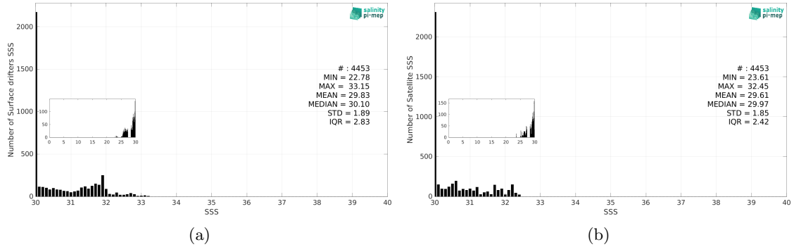
Figure 2: Histograms of SSS from Surface drifters (a) and SMOS SSS L3 v9 - 18 Days (CATDS-CEC-LOCEAN) (b) considering all match-up pairs per bins of 0.1 over the Bay of Bengal Pi-MEP region and for the full satellite product period.
