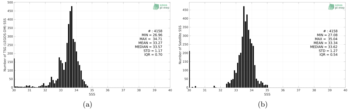
Figure 2: Histograms of SSS from TSG (LEGOS-DM) (a) and SMOS SSS L3 v8 - 9 Days (CATDS-CECOS-LOCEAN) (b) considering all match-up pairs per bins of 0.1 over the Bay of Bengal Pi-MEP region and for the full satellite product period.
