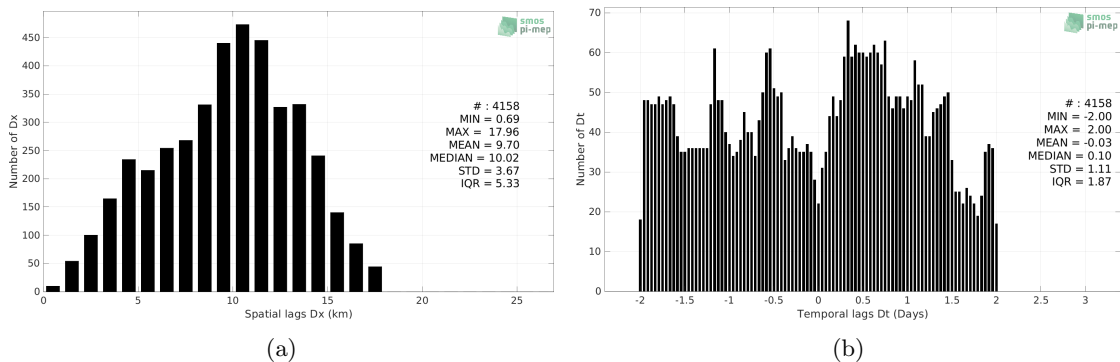
Figure 5: Histograms of the spatial (a) and temporal (b) lags between the location/time of the TSG (LEGOS-DM) measurement and the date of the corresponding SMOS SSS L3 v8 - 9 Days (CATDS-CECOS-LOCEAN) SSS pixel.
