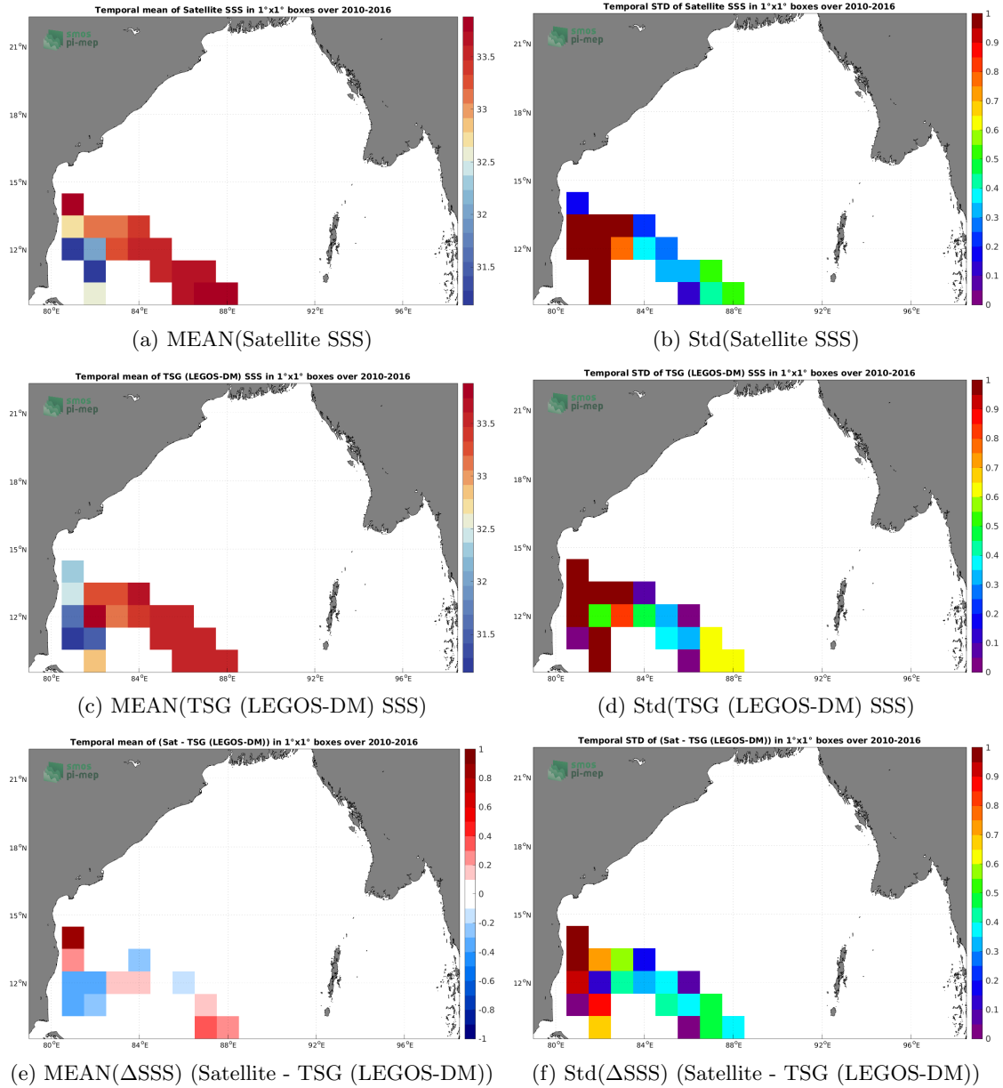
Figure 6: Temporal mean (left) and Std (right) of SSS from SMOS SSS L3 v8 - 9 Days (CATDS-CECOS-LOCEAN) (top), TSG (LEGOS-DM) (middle), and of \Delta SSS (Satellite - TSG (LEGOS-DM)). Only match-up pairs are used to generate these maps.
