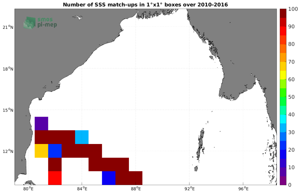
Figure 4: Number of SSS match-ups between TSG (LEGOS-DM) SSS and the SMOS SSS L3 v8 - 9 Days (CATDS-CECOS-LOCEAN) SSS product for the Bay of Bengal Pi-MEP region over 1^\circ \times 1^\circ boxes and for the full satellite product period.
