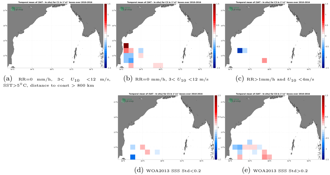
Figure 12: Temporal mean gridded over spatial boxes of size 1^{\circ}\times 1^{\circ} of \Delta\text{SSS} (SMOS SSS L3 v8 - 9 Days (CATDS-CECOS-LOCEAN) - TSG (LEGOS-DM)) for 5 different subdatasets corresponding to: RR=0 mm/h, 3 < U_{10} < 12 m/s, SST > 5^{\circ}\text{C} , distance to coast > 800 km (a), RR=0 mm/h, 3 < U_{10} < 12 m/s (b), RR > 1 mm/h and U_{10} < 4 m/s (c), WOA2013 SSS Std < 0.2 (d), WOA2013 SSS Std > 0.2 (e).
