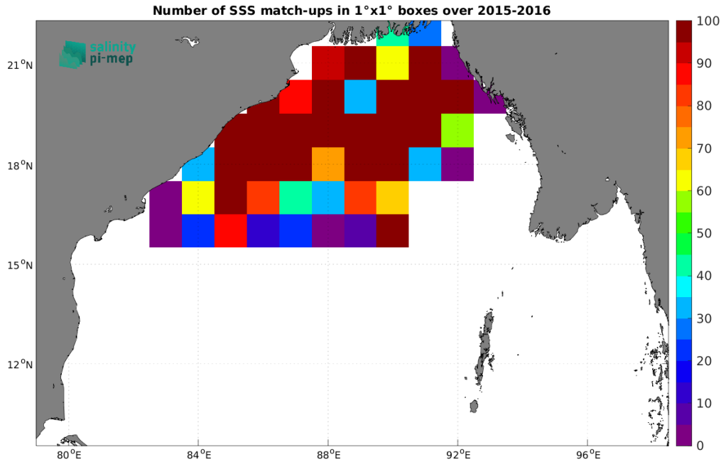
Figure 3: Number of SSS match-ups between Surface drifters SSS and the SMOS SSS L3 v8 - 9 Days (CATDS-CEC-LOCEAN) SSS product for the Bay of Bengal Pi-MEP region over 1^\circ \times 1^\circ boxes and for the full satellite product period.
