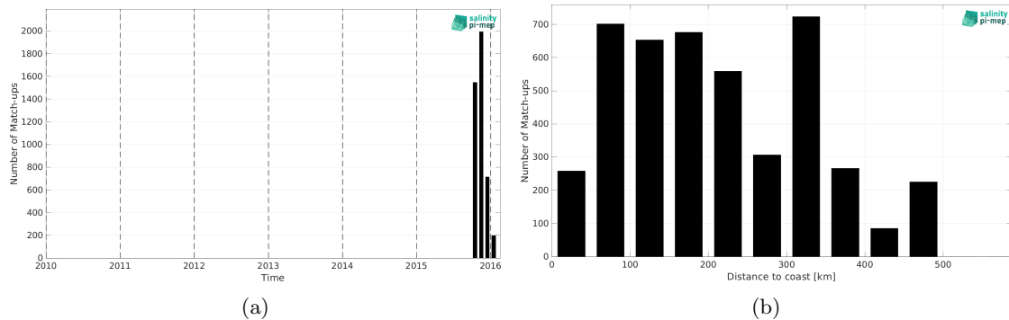
Figure 1: Number of match-ups between Surface drifters and SMOS SSS L3 v8 - 9 Days (CATDS-CEC-LOCEAN) SSS as a function of time (a) and as function of the distance to coast (b) over the Bay of Bengal Pi-MEP region and for the full satellite product period.
