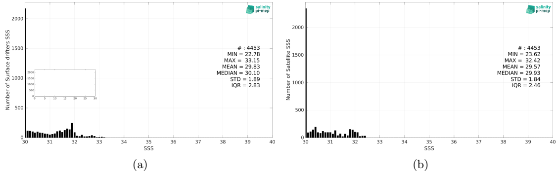
Figure 2: Histograms of SSS from Surface drifters (a) and SMOS SSS L3 v8 - 9 Days (CATDS-CEC-LOCEAN) (b) considering all match-up pairs per bins of 0.1 over the Bay of Bengal Pi-MEP region and for the full satellite product period.
