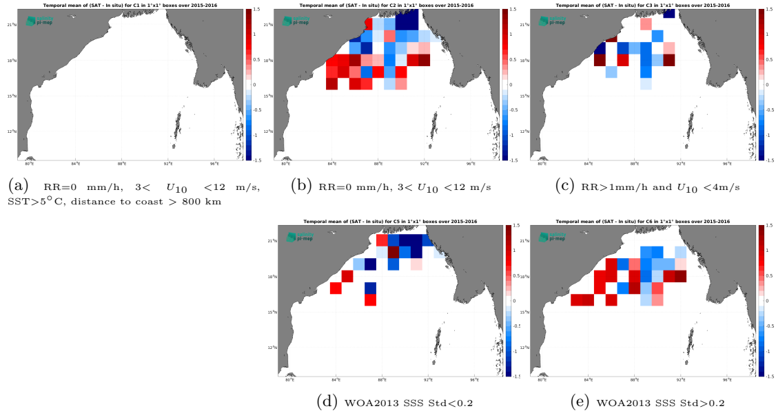
Figure 11: Temporal mean gridded over spatial boxes of size 1^{\circ}\times 1^{\circ} of \Delta\text{SSS} (SMOS SSS L3 v8 - 9 Days (CATDS-CEC-LOCEAN) - Surface drifters) for 5 different subdatasets corresponding to:RR=0 mm/h, 3 < U_{10} < 12 m/s, SST > 5^{\circ}\text{C} , distance to coast > 800 km (a), RR=0 mm/h, 3 < U_{10} < 12 m/s (b), RR > 1 mm/h and U_{10} < 4 m/s (c), WOA2013 SSS Std < 0.2 (d), WOA2013 SSS Std > 0.2 (e).
