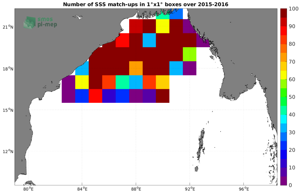
Figure 3: Number of SSS match-ups between Surface drifters SSS and the SMOS SSS L3 v8 - 9 Days (CATDS-CECOS-LOCEAN) SSS product for the Bay of Bengal Pi-MEP region over 1^\circ \times 1^\circ boxes and for the full satellite product period.
