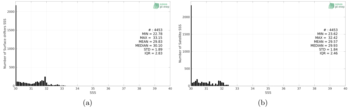
Figure 2: Histograms of SSS from Surface drifters (a) and SMOS SSS L3 v8 - 9 Days (CATDS-CECOS-LOCEAN) (b) considering all match-up pairs per bins of 0.1 over the Bay of Bengal Pi-MEP region and for the full satellite product period.
