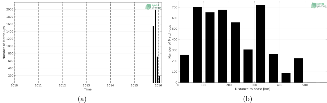
Figure 1: Number of match-ups between Surface drifters and SMOS SSS L3 v8 - 9 Days (CATDS-CECOS-LOCEAN) SSS as a function of time (a) and as function of the distance to coast (b) over the Bay of Bengal Pi-MEP region and for the full satellite product period.
