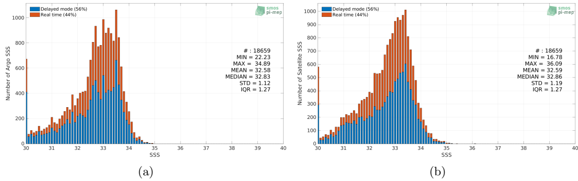
Figure 2: Histograms of SSS from Argo (a) and SMOS SSS L3 v8 - 9 Days (CATDS-CECOS-LOCEAN) (b) considering all match-up pairs per bins of 0.1 over the Bay of Bengal Pi-MEP region and for the full satellite product period.
