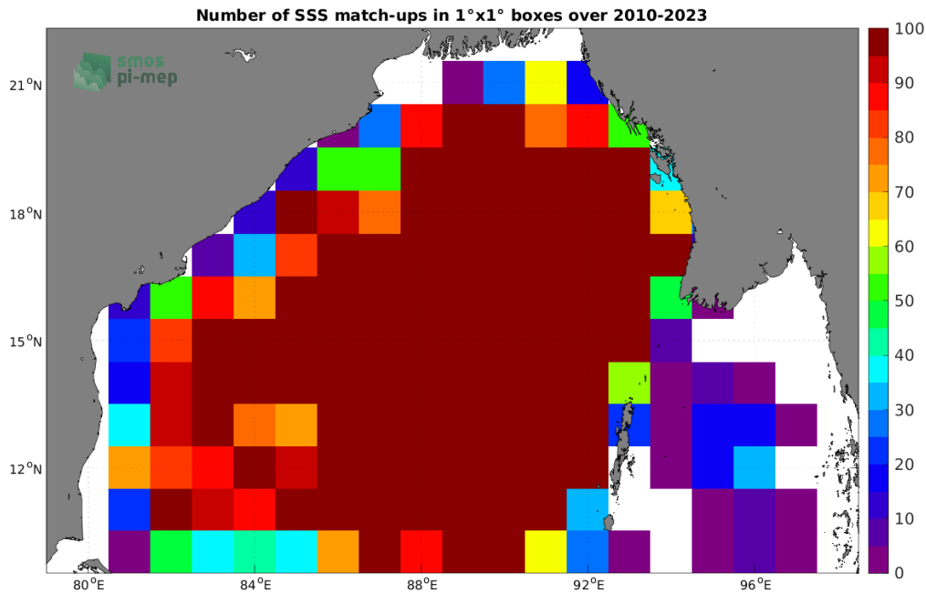
Figure 4: Number of SSS match-ups between Argo SSS and the SMOS SSS L3 v8 - 9 Days (CATDS-CECOS-LOCEAN) SSS product for the Bay of Bengal Pi-MEP region over 1^\circ \times 1^\circ boxes and for the full satellite product period.
