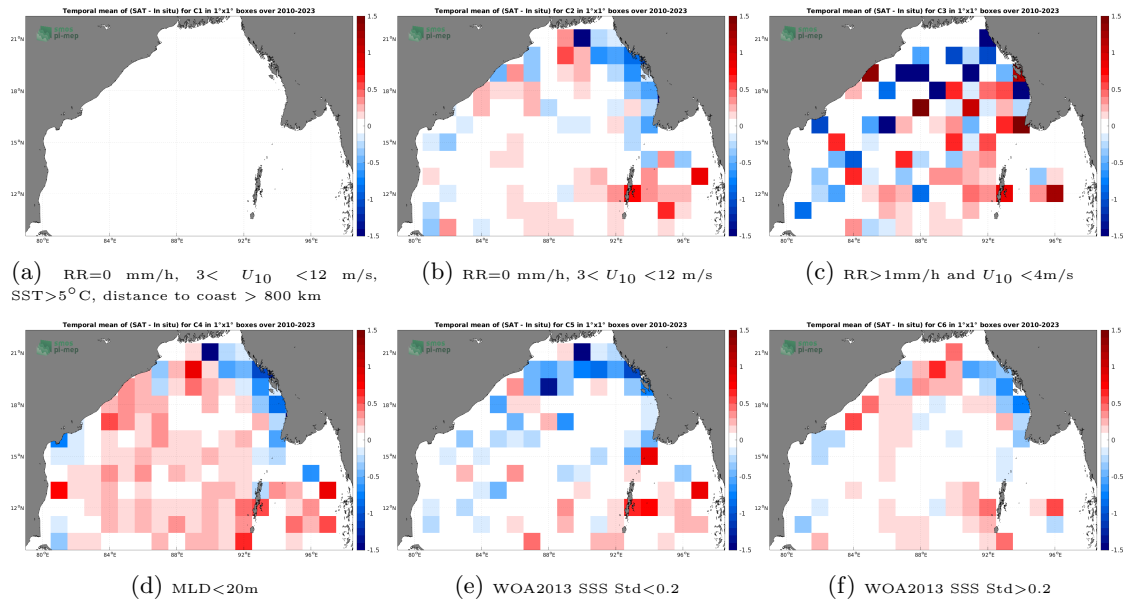
Figure 12: Temporal mean gridded over spatial boxes of size 1^\circ \times 1^\circ of \Delta SSS (SMOS SSS L3 v8 - 9 Days (CATDS-CECOS-LOCEAN) - Argo) for 6 different subdatasets corresponding to:RR=0 mm/h, 3 < U_{10} < 12 m/s, SST > 5^\circ\text{C} , distance to coast > 800 km (a), RR=0 mm/h, 3 < U_{10} < 12 m/s (b), RR > 1 mm/h and U_{10} < 4 m/s (c),MLD < 20 m (d),WOA2013 SSS Std < 0.2 (e),WOA2013 SSS Std > 0.2 (f).
