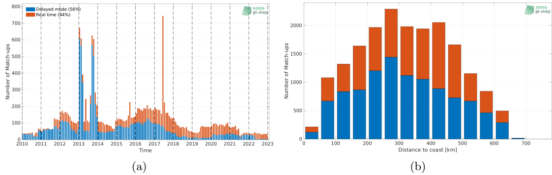
Figure 1: Number of match-ups between Argo and SMOS SSS L3 v8 - 9 Days (CATDS-CECOS-LOCEAN) SSS as a function of time (a) and as function of the distance to coast (b) over the Bay of Bengal Pi-MEP region and for the full satellite product period.
