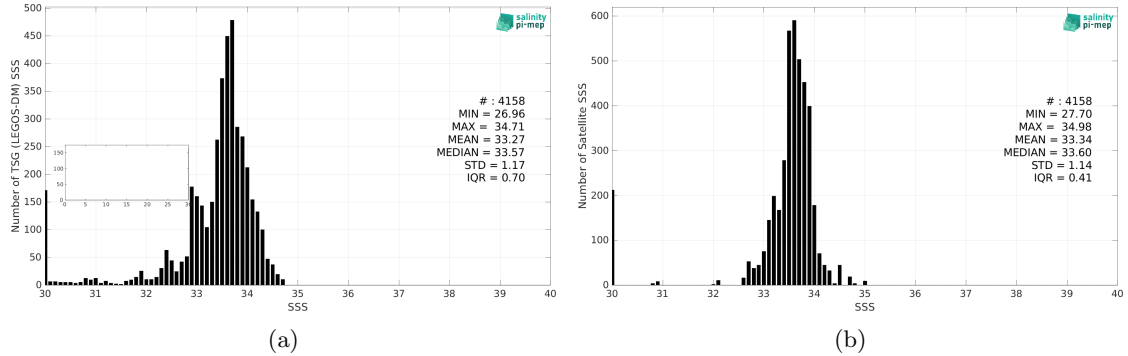
Figure 2: Histograms of SSS from TSG (LEGOS-DM) (a) and SMOS SSS L3 v8 - 18 Days (CATDS-CEC-LOCEAN) (b) considering all match-up pairs per bins of 0.1 over the Bay of Bengal Pi-MEP region and for the full satellite product period.
