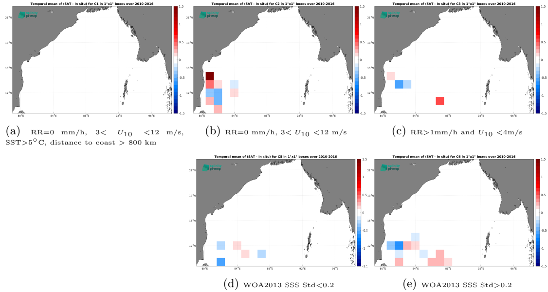
Figure 12: Temporal mean gridded over spatial boxes of size 1^{\circ}\times 1^{\circ} of \Delta\text{SSS} (SMOS SSS L3 v8 - 18 Days (CATDS-CEC-LOCEAN) - TSG (LEGOS-DM)) for 5 different subdatasets corresponding to: RR=0 mm/h, 3 < U_{10} < 12 m/s, SST > 5^{\circ}\text{C} , distance to coast > 800 km (a), RR=0 mm/h, 3 < U_{10} < 12 m/s (b), RR > 1 mm/h and U_{10} < 4 m/s (c), WOA2013 SSS Std < 0.2 (d), WOA2013 SSS Std > 0.2 (e).
