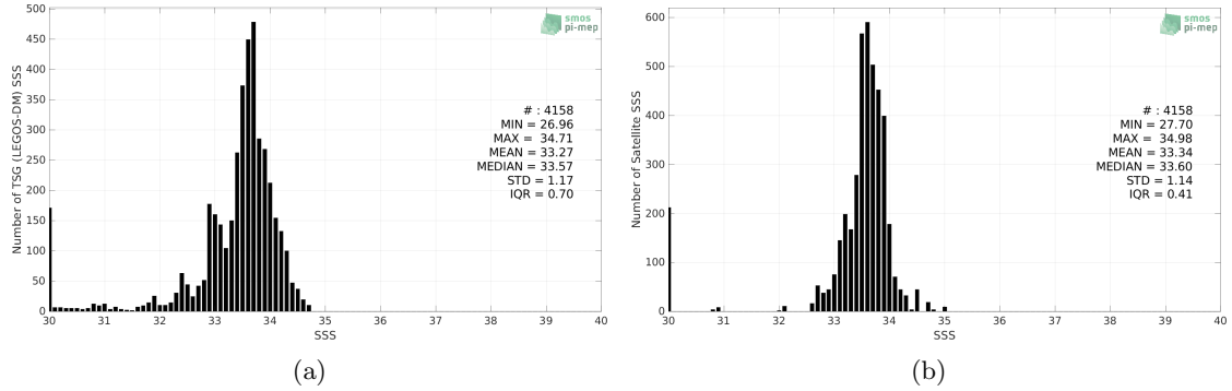
Figure 2: Histograms of SSS from TSG (LEGOS-DM) (a) and SMOS SSS L3 v8 - 18 Days (CATDS-CECOS-LOCEAN) (b) considering all match-up pairs per bins of 0.1 over the Bay of Bengal Pi-MEP region and for the full satellite product period.
