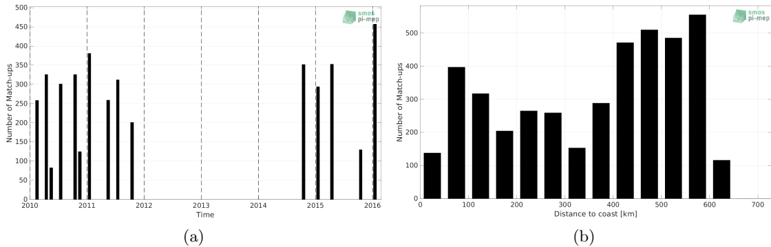
Figure 1: Number of match-ups between TSG (LEGOS-DM) and SMOS SSS L3 v8 - 18 Days (CATDS-CECOS-LOCEAN) SSS as a function of time (a) and as function of the distance to coast (b) over the Bay of Bengal Pi-MEP region and for the full satellite product period.
