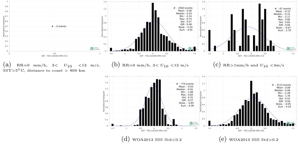
Figure 13: Normalized histogram of \Delta SSS (SMOS SSS L3 v8 - 18 Days (CATDS-CECOS-LOCEAN) - TSG (LEGOS-DM)) for 5 different subdatasets corresponding to: RR=0 mm/h, 3 < U_{10} < 12 m/s, SST > 5°C, distance to coast > 800 km (a), RR=0 mm/h, 3 < U_{10} < 12 m/s (b), RR > 1mm/h and U_{10} < 4 m/s (c), WOA2013 SSS Std < 0.2 (d), WOA2013 SSS Std > 0.2 (e).
