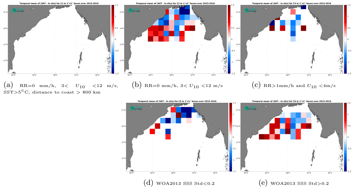
Figure 11: Temporal mean gridded over spatial boxes of size 1^{\circ}\times 1^{\circ} of \Delta\text{SSS} (SMOS SSS L3 v8 - 18 Days (CATDS-CEC-LOCEAN) - Surface drifters) for 5 different subdatasets corresponding to:RR=0 mm/h, 3 < U_{10} < 12 m/s, SST > 5^{\circ}\text{C} , distance to coast > 800 km (a), RR=0 mm/h, 3 < U_{10} < 12 m/s (b), RR > 1 mm/h and U_{10} < 4 m/s (c), WOA2013 SSS Std < 0.2 (d), WOA2013 SSS Std > 0.2 (e).
