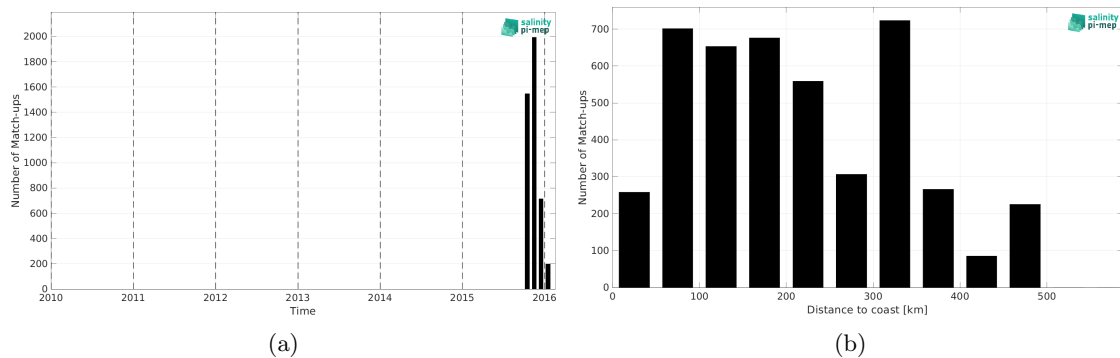
Figure 1: Number of match-ups between Surface drifters and SMOS SSS L3 v8 - 18 Days (CATDS-CEC-LOCEAN) SSS as a function of time (a) and as function of the distance to coast (b) over the Bay of Bengal Pi-MEP region and for the full satellite product period.
