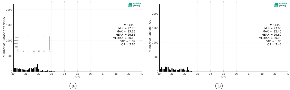
Figure 2: Histograms of SSS from Surface drifters (a) and SMOS SSS L3 v8 - 18 Days (CATDS-CEC-LOCEAN) (b) considering all match-up pairs per bins of 0.1 over the Bay of Bengal Pi-MEP region and for the full satellite product period.
