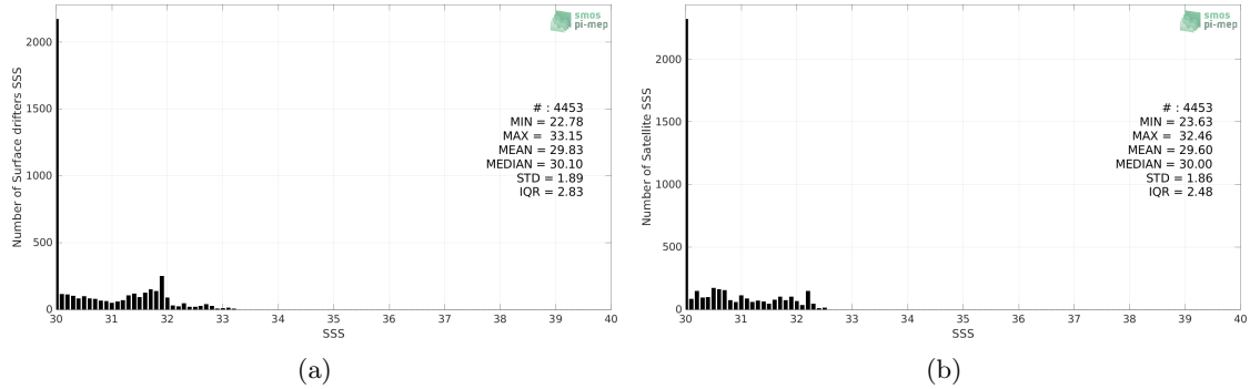
Figure 2: Histograms of SSS from Surface drifters (a) and SMOS SSS L3 v8 - 18 Days (CATDS-CECOS-LOCEAN) (b) considering all match-up pairs per bins of 0.1 over the Bay of Bengal Pi-MEP region and for the full satellite product period.
