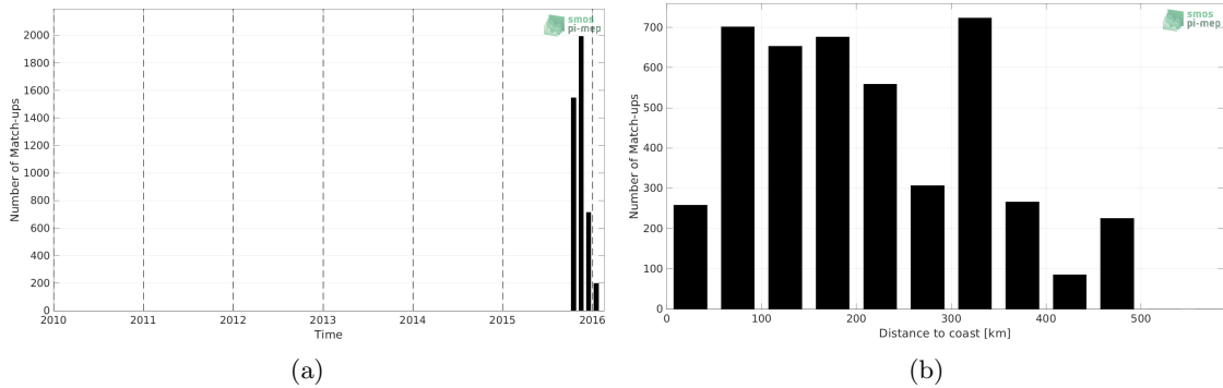
Figure 1: Number of match-ups between Surface drifters and SMOS SSS L3 v8 - 18 Days (CATDS-CECOS-LOCEAN) SSS as a function of time (a) and as function of the distance to coast (b) over the Bay of Bengal Pi-MEP region and for the full satellite product period.
