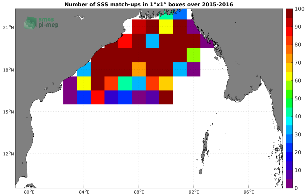
Figure 3: Number of SSS match-ups between Surface drifters SSS and the SMOS SSS L3 v8 - 18 Days (CATDS-CECOS-LOCEAN) SSS product for the Bay of Bengal Pi-MEP region over 1^\circ \times 1^\circ boxes and for the full satellite product period.
