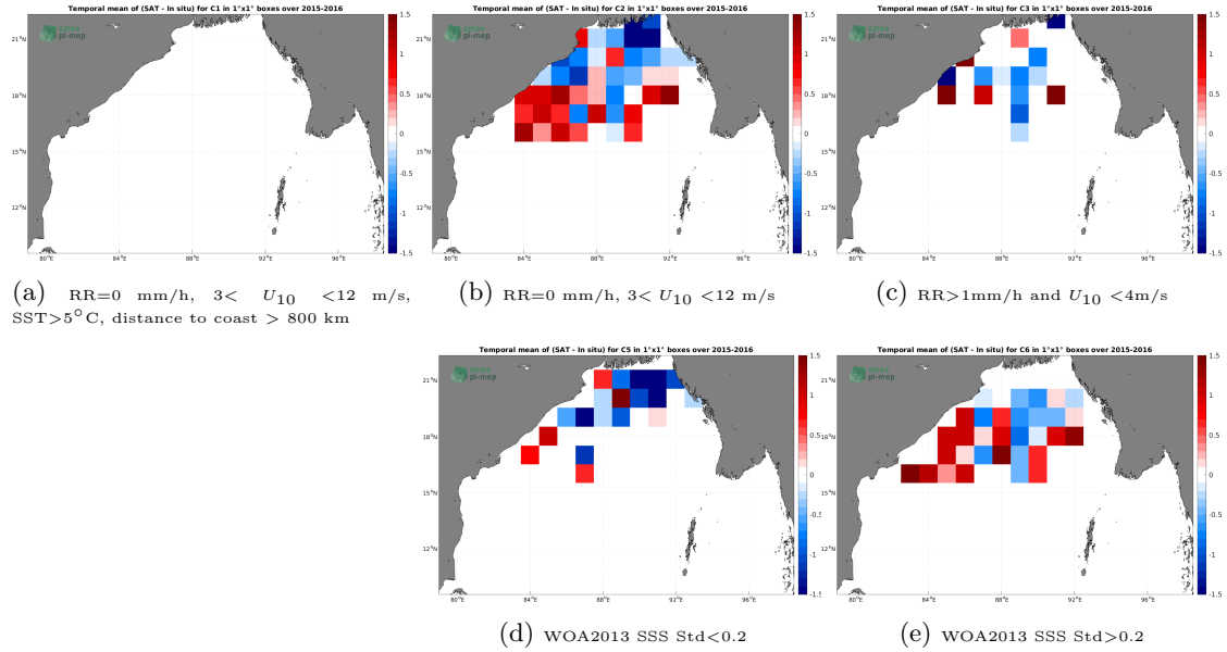
Figure 11: Temporal mean gridded over spatial boxes of size 1^{\circ}\times 1^{\circ} of \Delta\text{SSS} (SMOS SSS L3 v8 - 18 Days (CATDS-CECOS-LOCEAN) - Surface drifters) for 5 different subdatasets corresponding to:RR=0 mm/h, 3 < U_{10} < 12 m/s, SST > 5^{\circ}\text{C} , distance to coast > 800 km (a), RR=0 mm/h, 3 < U_{10} < 12 m/s (b), RR > 1 mm/h and U_{10} < 4 m/s (c), WOA2013 SSS Std < 0.2 (d), WOA2013 SSS Std > 0.2 (e).
