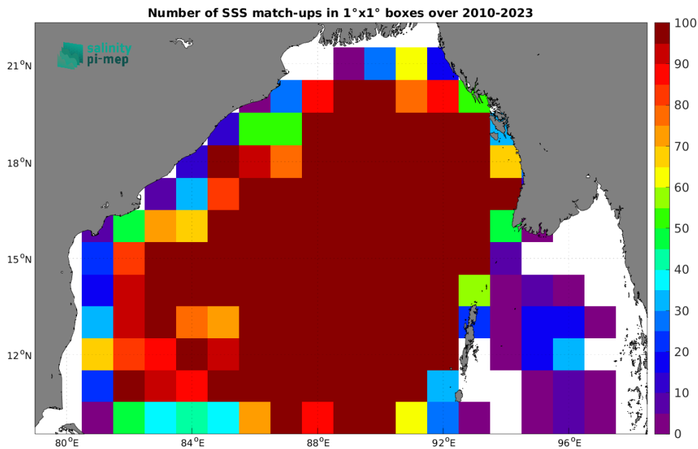
Figure 4: Number of SSS match-ups between Argo SSS and the SMOS SSS L3 v8 - 18 Days (CATDS-CEC-LOCEAN) SSS product for the Bay of Bengal Pi-MEP region over 1^\circ \times 1^\circ boxes and for the full satellite product period.
