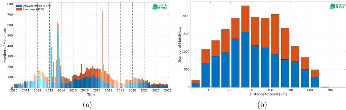
Figure 1: Number of match-ups between Argo and SMOS SSS L3 v8 - 18 Days (CATDS-CEC-LOCEAN) SSS as a function of time (a) and as function of the distance to coast (b) over the Bay of Bengal Pi-MEP region and for the full satellite product period.
