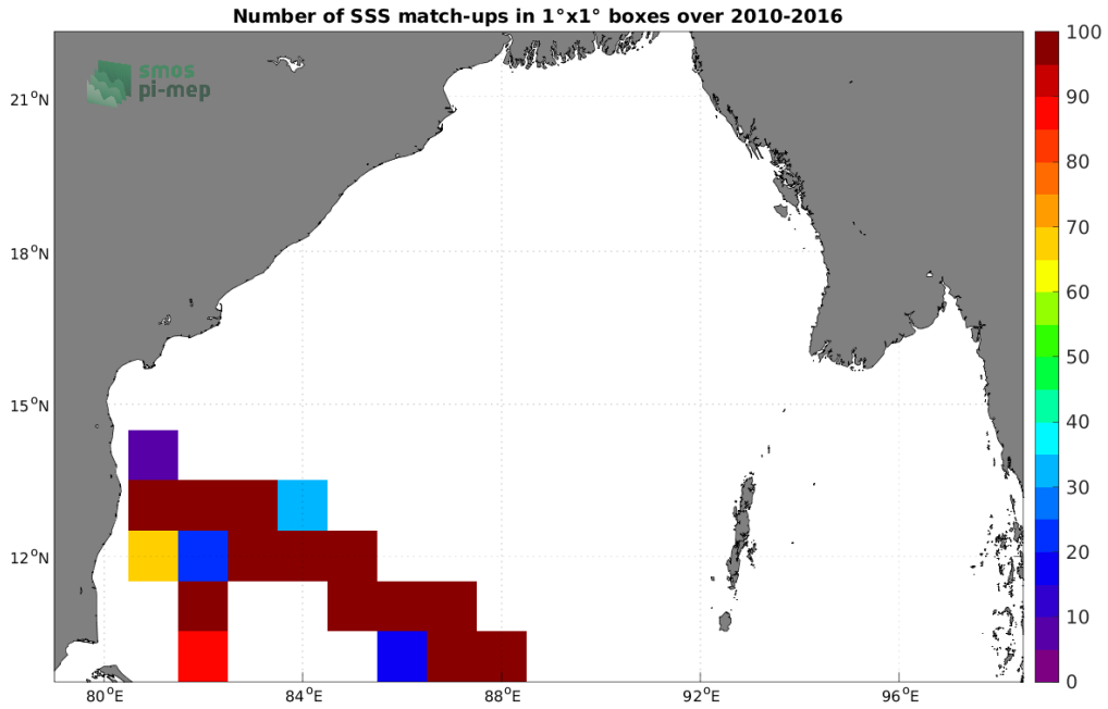
Figure 4: Number of SSS match-ups between TSG (LEGOS-DM) SSS and the SMOS SSS L3 v7 - 9 Days (CATDS-CECOS-LOCEAN) SSS product for the Bay of Bengal Pi-MEP region over 1°x1° boxes and for the full satellite product period.
