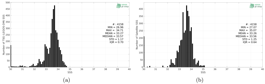
Figure 2: Histograms of SSS from TSG (LEGOS-DM) (a) and SMOS SSS L3 v7 - 9 Days (CATDS-CECOS-LOCEAN) (b) considering all match-up pairs per bins of 0.1 over the Bay of Bengal Pi-MEP region and for the full satellite product period.
