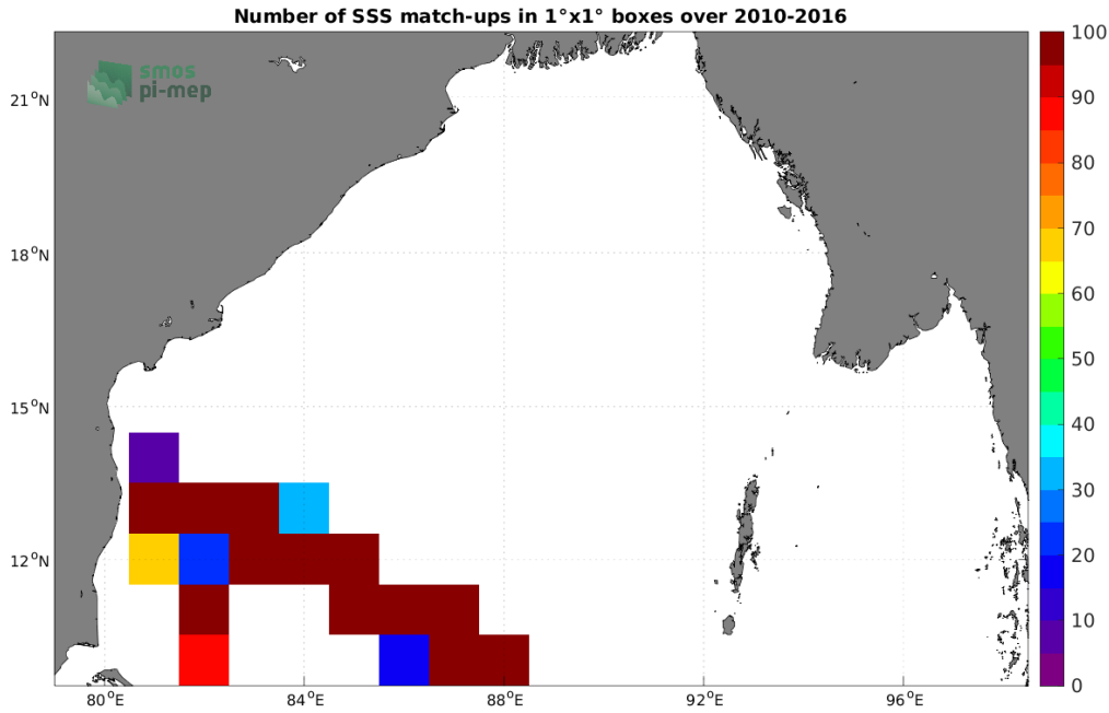
Figure 4: Number of SSS match-ups between TSG (LEGOS-DM) SSS and the SMOS SSS L3 v7 - 9 Days (CATDS-CECOS-LOCEAN) SSS product for the Bay of Bengal Pi-MEP region over 1^\circ \times 1^\circ boxes and for the full satellite product period.
