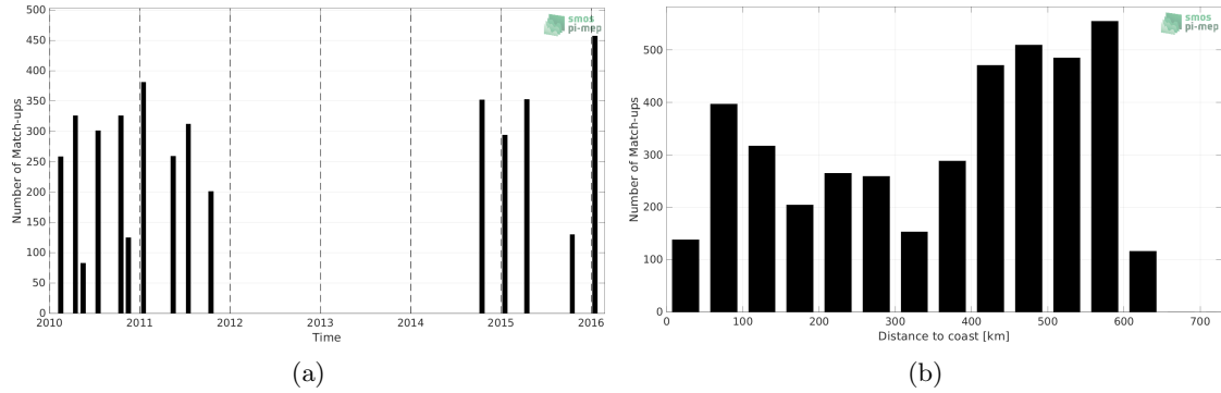
Figure 1: Number of match-ups between TSG (LEGOS-DM) and SMOS SSS L3 v7 - 9 Days (CATDS-CECOS-LOCEAN) SSS as a function of time (a) and as function of the distance to coast (b) over the Bay of Bengal Pi-MEP region and for the full satellite product period.
