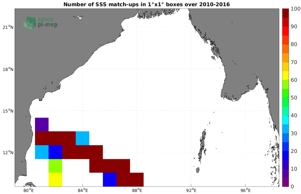
Figure 4: Number of SSS match-ups between TSG (LEGOS-DM) SSS and the SMOS SSS L3 v7 - 18 Days (CATDS-CECOS-LOCEAN) SSS product for the Bay of Bengal Pi-MEP region over 1^\circ \times 1^\circ boxes and for the full satellite product period.
