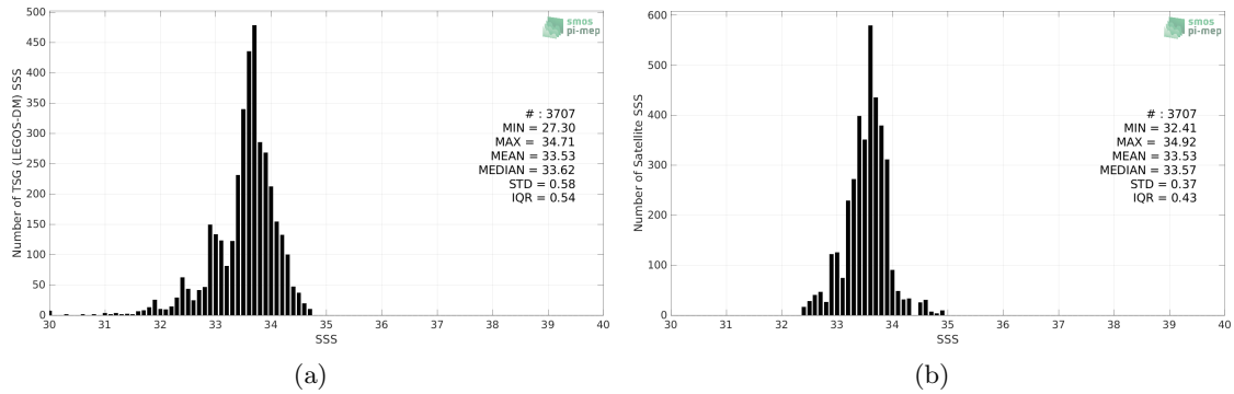
Figure 2: Histograms of SSS from TSG (LEGOS-DM) (a) and SMOS SSS L3 v7 - 18 Days (CATDS-CECOS-LOCEAN) (b) considering all match-up pairs per bins of 0.1 over the Bay of Bengal Pi-MEP region and for the full satellite product period.
