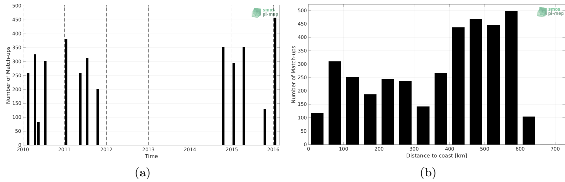
Figure 1: Number of match-ups between TSG (LEGOS-DM) and SMOS SSS L3 v7 - 18 Days (CATDS-CECOS-LOCEAN) SSS as a function of time (a) and as function of the distance to coast (b) over the Bay of Bengal Pi-MEP region and for the full satellite product period.
