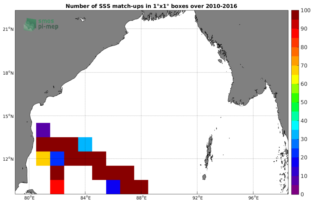
Figure 4: Number of SSS match-ups between TSG (LEGOS-DM) SSS and the SMOS SSS L3 v7 - 18 Days (CATDS-CECOS-LOCEAN) SSS product for the Bay of Bengal Pi-MEP region over 1^{\circ} \times 1^{\circ} boxes and for the full satellite product period.
