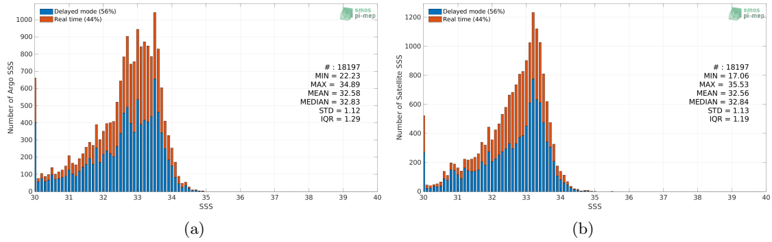
Figure 2: Histograms of SSS from Argo (a) and SMOS SSS L3 v7 - 18 Days (CATDS-CECOS-LOCEAN) (b) considering all match-up pairs per bins of 0.1 over the Bay of Bengal Pi-MEP region and for the full satellite product period.
