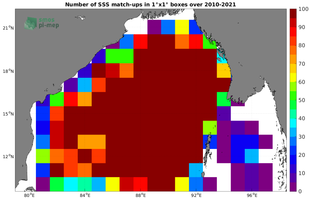
Figure 4: Number of SSS match-ups between Argo SSS and the SMOS SSS L3 v7 - 18 Days (CATDS-CECOS-LOCEAN) SSS product for the Bay of Bengal Pi-MEP region over 1^{\circ} \times 1^{\circ} boxes and for the full satellite product period.
