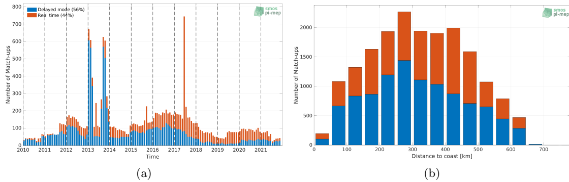
Figure 1: Number of match-ups between Argo and SMOS SSS L3 v7 - 18 Days (CATDS-CECOS-LOCEAN) SSS as a function of time (a) and as function of the distance to coast (b) over the Bay of Bengal Pi-MEP region and for the full satellite product period.
