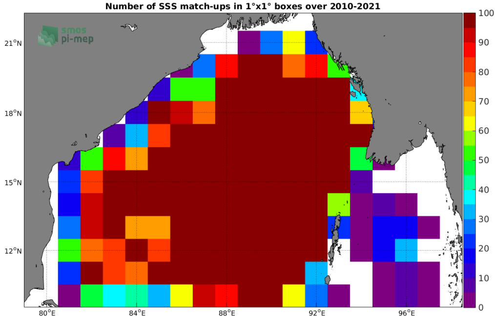
Figure 4: Number of SSS match-ups between Argo SSS and the SMOS SSS L3 v7 - 18 Days (CATDS-CECOS-LOCEAN) SSS product for the Bay of Bengal Pi-MEP region over 1^\circ \times 1^\circ boxes and for the full satellite product period.
